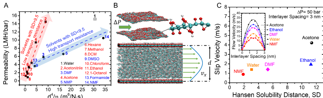
Figure 5. Mechanisms of solvent transport in GO membrane. The effect of solvent properties ( d^4/\eta ) and Hansen solubility distance (SD) on the permeability of solvents through GO membrane (A). Schematic illustration of molecular dynamics modeling of solvents transport between two parallel GO nanosheets under a transmembrane pressure of \Delta P (B). The interlayer spacing of the modelled GO nanosheets is fixed at 3 nm. The effect of Hansen solubility distance (SD) on the slip velocity of selected solvents (C). The insertion illustrates the representative flow velocity profiles of different solvents in the GO channel.
