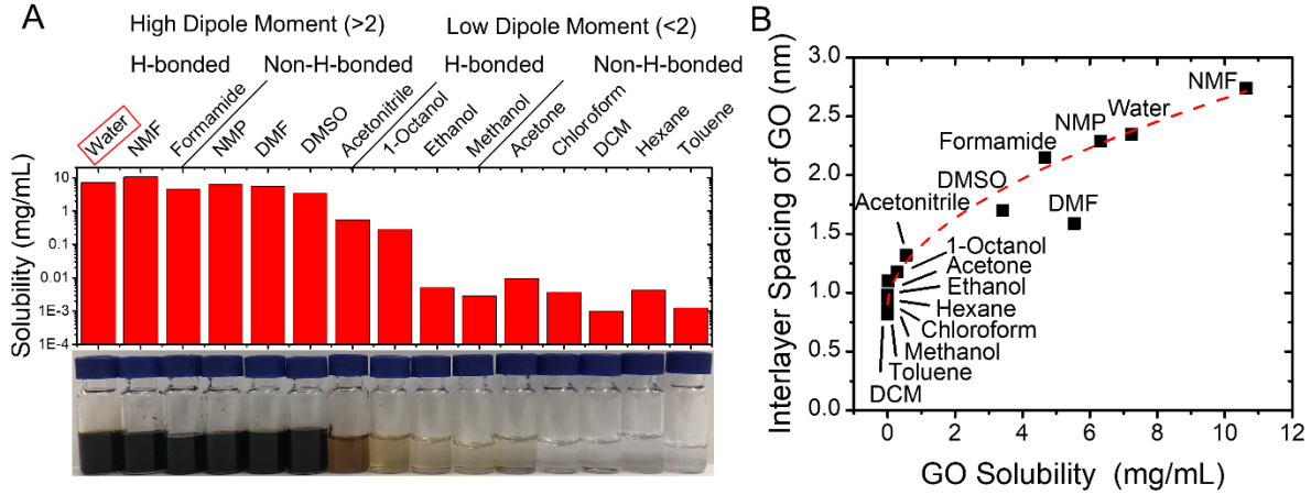
Figure 3. The experimentally measured solubility of GO in selected solvents (A), and its strong correlation with the interlayer spacing of GO obtained from ellipsometry measurements (B).
