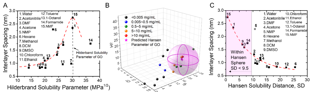
Figure 4. Prediction of swelling/interlayer spacing of GO based on solubility parameters. Correlation between the interlayer spacing of GO and the Hildebrand solubility parameter (A). Illustration of the Hansen space based on the Hansen solubility parameters of solvents and the predicted values of GO (B). Hansen sphere is represented by the pink sphere with a center at GO (pink star) and a radius of 9.5. The solvents with Hansen Solubility Distance (SD) < 9.5 are located within the Hansen sphere, and the solvents with SD > 9.5 are located outside of the Hansen sphere. Correlation between the interlayer spacing of GO in different solvents and their Hansen solubility distance, SD (C).
