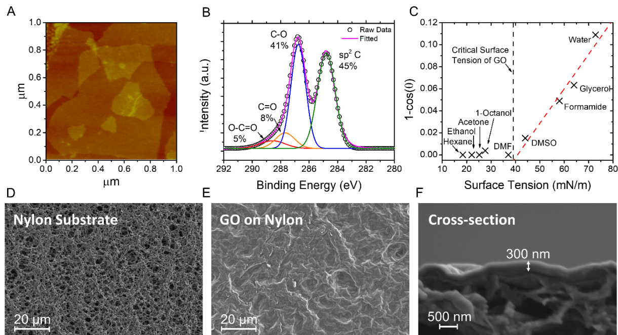
Figure 1. Physicochemical properties of GO nanosheets and layer-stacked GO membrane. AFM image of the as-synthesized GO nanosheets with a depth profile analysis demonstrating a monolayer thickness of around 1 nm (A). XPS characterization of the as-synthesized GO nanosheets confirming the abundance of oxygenated functional groups (B). The Zisman plot to extrapolate the critical surface tension of GO (DMSO denotes for dimethyl sulfoxide) (C). The SEM images of the top surface of the bare Nylon substrate (D), the top surface of GO membrane (E), and the cross section of GO membrane (F).
