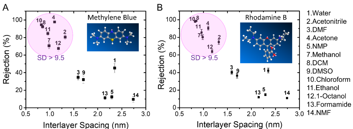
Figure 6. Rejection of methylene blue (A) and rhodamine B (B) by GO membrane in different organic solvents. The feed solution contains 100 ppm methylene blue or rhodamine B. Inserted are the chemical structures of methylene blue and rhodamine B.
