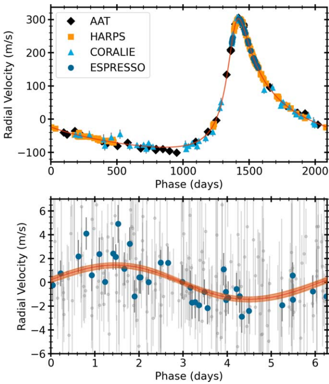
Figure 11. Radial velocity data phase-folded to the orbital periods of \pi Men b (top panel) and \pi Men c (bottom panel). The bottom panel shows the RV data with the contribution from the other planet removed.
