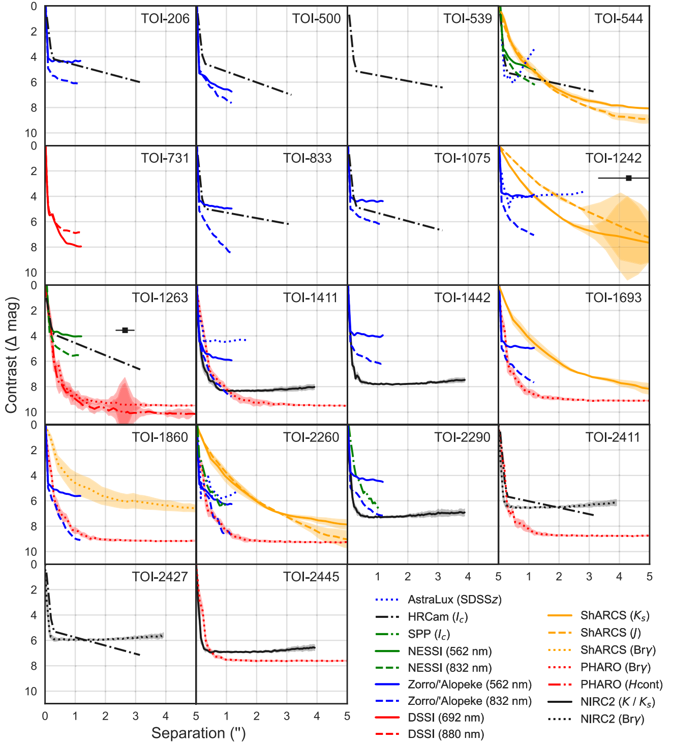
Figure 2. Contrast curves extracted from the high-resolution follow-up observations summarized in Table 4, which allows us to rule out companions at a given separation above a certain \Delta mag. Curves without shading (i.e., those from lucky and speckle imaging) were constructed by taking the 5\sigma upper limits of the contrasts in circular annuli around the target star. Curves with shading (i.e., those from adaptive optics imaging) were constructed by taking the mean and rms error of the contrasts in circular annuli around the target star. TOI-1242 and TOI-1263 have <5'' companions, which are both known stars in the TIC. The TESS band \Delta mag and separations of these companions are indicated by black squares. These curves are folded into the TRICERATOPS analysis described in Section 3.
