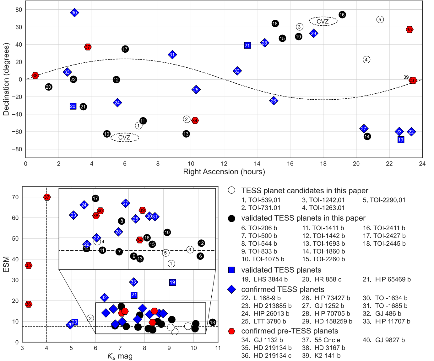
Figure 12. Top: coordinates of the TESS planet candidates in this paper (white circles), validated TESS planets in this paper (black circles), validated TESS planets (blue squares), confirmed TESS planets (blue diamonds), and confirmed pre-TESS planets (red hexagons). The ecliptic plane and ecliptic poles (i.e., the JWST continuous viewing zones) are shown as dashed black lines. Bottom: emission spectroscopy metric versus apparent K_s magnitude for each planet candidate and planet. The dashed lines indicate the minimum values a target should have to be observed with JWST.
