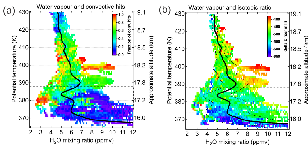
Figure 4. Binned ensemble (bin size 0.1 ppmv by 1 K) of FLASH H 2 O measurements from all flights except F1 and F5 for which no isotopic data are available. The pixels are colour-coded by (a) convective hits fraction (see text for details) and (b) the ChiWIS HDO/H 2 O isotopic ratio. The black solid and dashed curves depict campaign-median H 2 O profile and 1 standard deviation respectively (all flights). The horizontal dashed lines mark the vertical range of the CPT level encountered during the campaign. Note that the convective origin is specific to both anomalously wet and anomalously dry parcels (a), whereas the wettest parcels in the lower stratosphere are isotopically enhanced (b).
