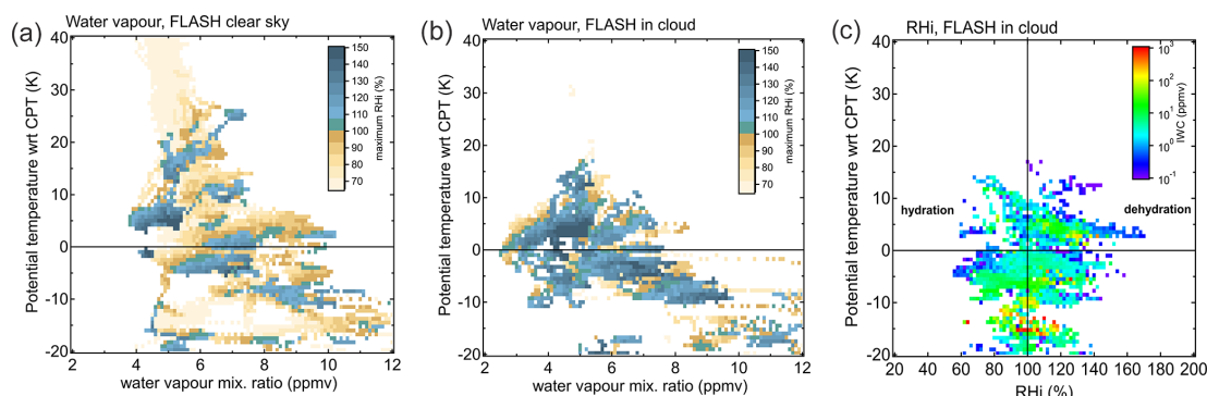
Figure 3. (a, b) Binned distribution of maximum RHi (computed from FLASH and TDC measurements) as a function of FLASH water vapour and potential temperature relative to the local CPT level (bin size 0.1 ppmv by 1 K) for (a) clear-sky conditions and (b) cloud occurrence detected by MAS (see Sect. 2.1.2). (c) Binned distribution of ice water content (IWC) exceeding 0.1 ppmv from NIXE-CAPS instrument inside clouds detected by MAS as a function of relative humidity over ice (RHi) and potential temperature relative to the local CPT level. The presence of ice crystals in subsaturated air ( \text{RHi} < 100\% ) above the cold point tropopause potentially leads to permanent hydration of the CLS, whereas in supersaturated air the ice crystals are expected to sediment out of the CLS, thereby leading to its dehydration.
