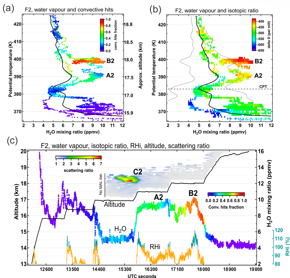
Figure 6. Results of F2 measurements (29 July) with the features of interest marked A2, B2 and C2. (a) Water vapour profile (FLASH) colour-coded by convective hits density (see text for details). (b) Same as panel (a) but colour-coded by the ChiWIS HDO/H 2 O isotopic ratio. The black solid and dashed curves depict the campaign-median H 2 O profile and 2 standard deviations respectively. (c) Time series of flight altitude (black curve), water vapour (colour-coded by convective hits density) and RH (right-hand axis) computed from FLASH and TDC measurements. The colour map shows the scattering ratio measured by MAL (upward-looking).
