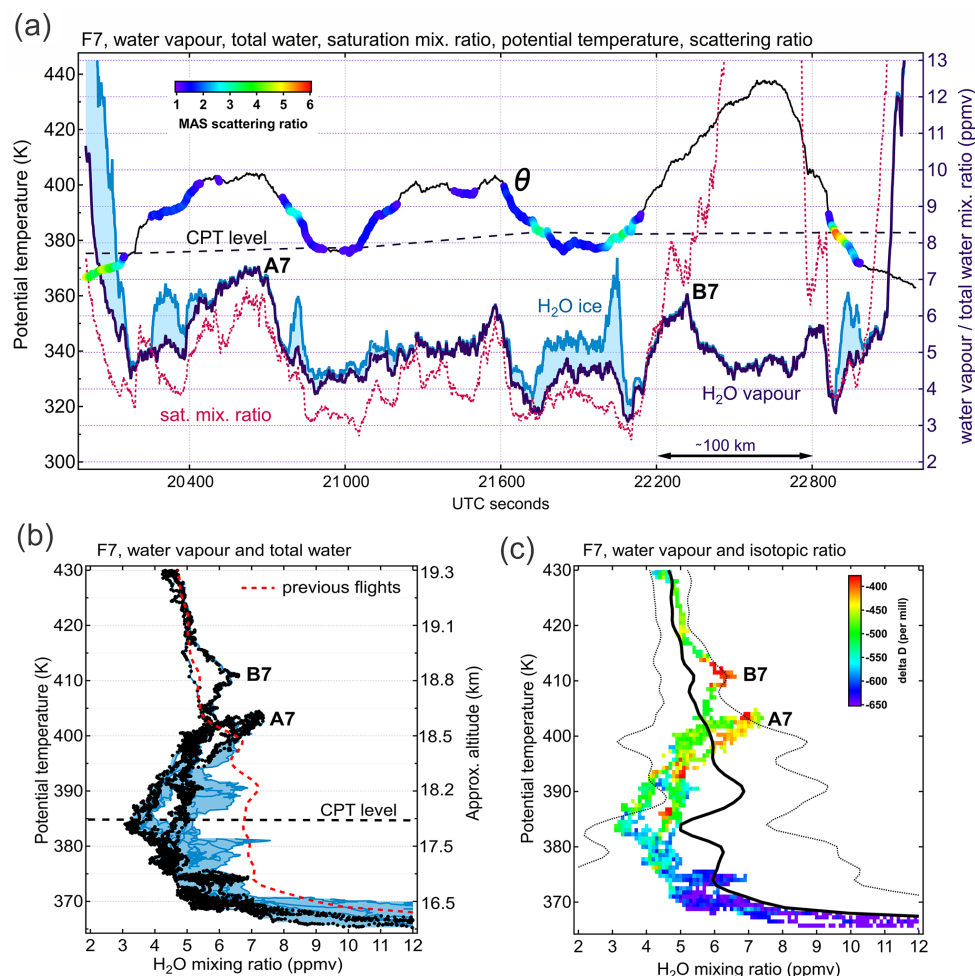
Figure 8. Results of F7 measurements (8 August) with the features of interest marked A7 and B7. (a) Time series of potential temperature \theta (left-hand axis) and water vapour/total water (right-hand axis). The \theta time series is tagged by cloud occurrence and colour-coded by the scattering ratio. The IWC is shown as cyan shading stacked on the water vapour curve, and the darker cyan curve depicts the total water (right-hand axis). The dashed magenta line depicts the saturation mixing ratio (right-hand axis). The CPT level displayed as the black dashed line is inferred from airborne measurements. (b) Vertical profiles of water vapour (black circles), total water (cyan) and IWC (cyan shading). The red dashed curve indicates the mean water vapour profile from the previous flights (F1–F6). (c) Binned water vapour profile with pixels colour-coded by the HDO/H 2 O isotopic ratio. The black solid curve depicts the campaign-median H 2 O profile, and the dotted curves represent 2 standard deviations respectively.
