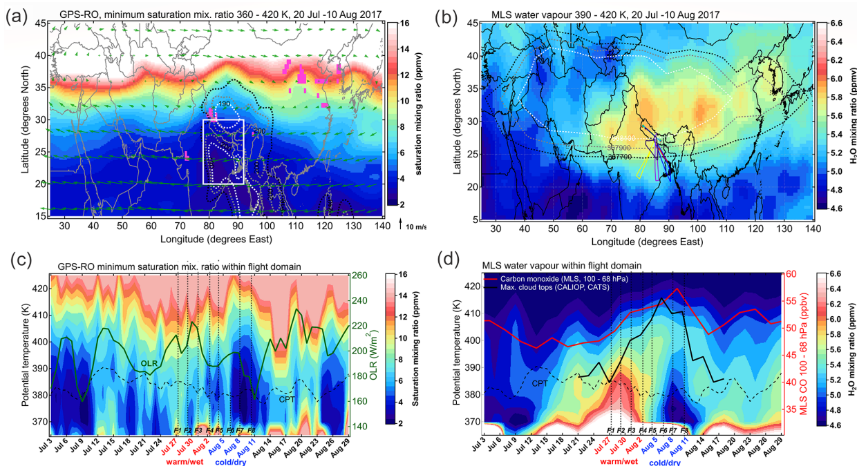
Figure 1. Overview and evolution of AMA UTLS conditions during July–August 2017 from satellite observations. (a) Colour map shows the GPS-RO minimum saturation mixing ratio (ppmv) encountered within the 360–420 K layer during the 20 July–10 August 2017 period. Dashed contours indicate National Centers for Environmental Prediction (NCEP) OLR ( \text{W m}^{-2} ) in the range 190–210 \text{W m}^{-2} (contour interval 10 \text{W m}^{-2} ). Green arrows are wind velocity vectors (ERA5, 70–100 hPa average for the campaign period). Pink pixels mark the most probable sources of the hydrated features (see Sect. 4.2). White rectangle indicates the flight domain. (b) Horizontal distribution of MLS water vapour in the confined LS (390–420 K layer) averaged over the 20 July–10 August period with the date-coloured flight tracks superimposed (see Fig. 2 for colour definition). Dashed contours depict the Montgomery stream function ( \text{m}^{-2} \text{s}^{-2} ), which is used to define the horizontal boundaries of the AMA at 390–410 K levels (Santee et al., 2016). (c) Evolution of the GPS-RO minimum saturation mixing ratio profile within the flight domain (20–30° N, 78–92° E). Green curve plotted versus right-hand axis depicts the domain-mean OLR. (d) Evolution of the MLS water vapour profile within the flight domain. The solid black curve depicts the maximum level of cloud tops detected using CALIOP and CATS satellite lidars. The red curve indicates MLS carbon monoxide (68–100 hPa mean). The vertical dashed lines indicate the flight dates (flight number is given as Fx) and their vertical extent, and the dashed curve marks the average CPT potential temperature level (GPS-RO) in both panels (c) and (d).
