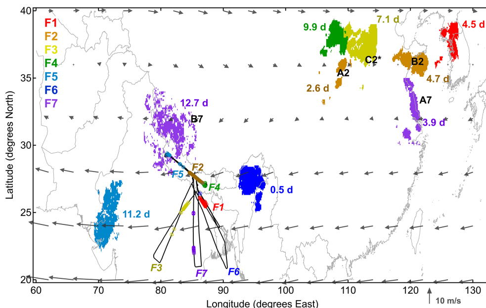
Figure 5. Composite map of convective clouds (highest cloud class) linked by back trajectories with the observed hydrated (wet-and-heavy) parcels. The colour of convective systems indicates the flight number (F x ; see legend) in which the respective parcels were sampled. The same colour code is used to mark the flight segments where these parcels were probed. The convective age (days) is indicated for each convective system. The convective sources for the features of interest in flight F2 (A2, B2, C2*) and F7 (A7, B7) are annotated (see Sect. 5). The arrows are wind velocity vectors (ERA5, 70–100 hPa average).
