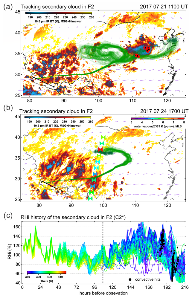
Figure 7. Trajectory analysis of the secondary cloud (C2) detected in F2 (29 July). (a) Back trajectories (green curves) and convective hits locations (black-filled red circles) superimposed onto the infrared brightness temperature (IR BT) at the time of convective hits (cf. time stamp in the panel). (b) Same as panel (a) but for the time of the MLS sampling of the moist plume. The spatiotemporally collocated MLS swath is displayed as markers colour-coded by the H 2 O mixing ratio at the 393 K level. The wettest MLS measurement coincides with the location of hydrated parcels. (c) Relative humidity over ice evolution along the back trajectories with colour coding by potential temperature computed from ERA5 temperature and assumed H 2 O mixing ratio of 12 ppmv (see text for details). The black markers show the locations of convective hits, and the vertical dashed line indicates the time of MLS sampling of the moist plume on 24 July.
