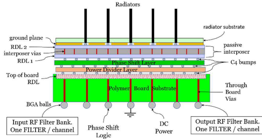
Figure 16. Cross sectional sketch of a 2.5D component stack-up process leading to an initial testable prototype.
