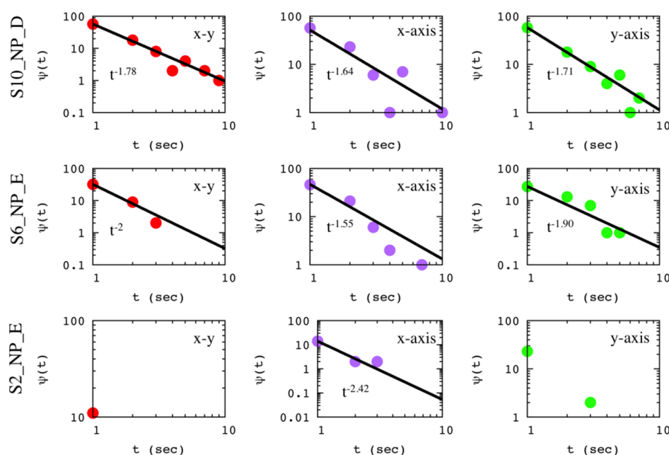
Figure 3. Waiting times distribution \psi(t) versus the elapse time t for three representative examples. Color code: red for the lateral motion of a micelle, purple for the motion in the x axis, and green for the motion in the y axis.
