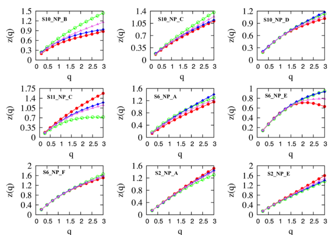
Figure 5. Structure functions for motion in x , y axes; red for z_{x,x} and green for z_{y,y} . In blue, the cross-correlation of movements in x and y axes. In violet, the theoretical value of the cross-correlation z_{x,y}^{theor}(q) = (z_{x,x}(q) + z_{y,y}(q))/2 . Notice that z_{\theta,\theta}(q) is not illustrated because it takes zero values for all q 's.
