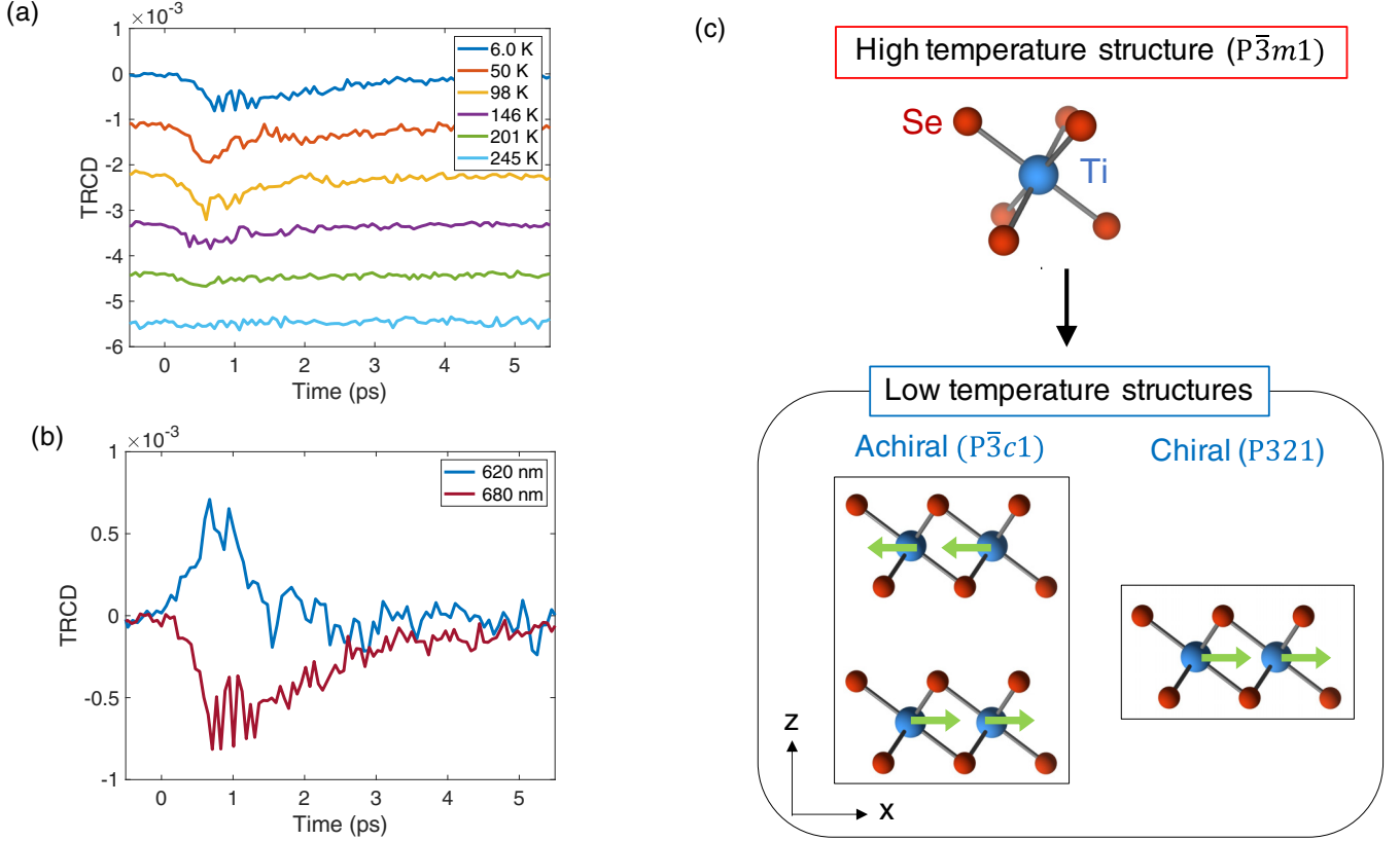
FIG. 1. Transient circular dichroism (TRCD) where \text{TRCD} = R_i^r(\lambda) - R_i^l(\lambda) measured on the picosecond timescale (a) as a function of temperature using a 680 nm probe wavelength and (b) measured at T = 7.6 K for 620 nm probe and T = 6.0 K for 680 nm probe. (c) Schematic depiction of how the achiral centrosymmetric high-temperature P\bar{3}m1 structure can transform into either the achiral centrosymmetric P\bar{3}c1 CDW structure or the chiral noncentrosymmetric P321 CDW structure as the temperature, T , is lowered below the CDW transition temperature. The green arrows indicate the direction that the Ti atoms are displaced in the CDW phase.
