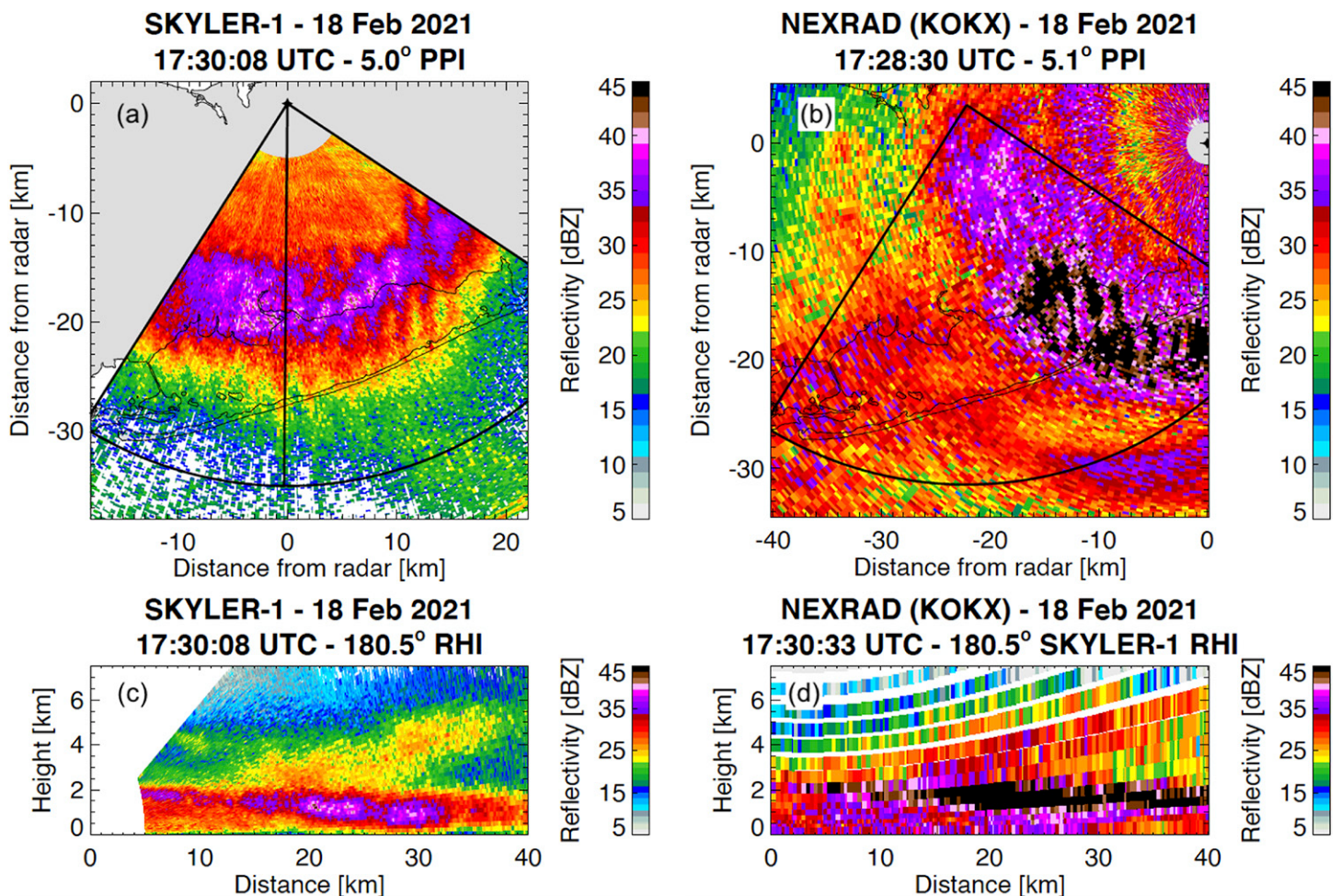
Fig. 3. (a) Example PPI at 5° from a winter storm on 18 Feb 2021 at 1730:08 UTC in Long Island, NY, from the Raytheon SKYLER-1 system (Kollias et al. 2022) at Stony Brook University; (b) the corresponding PPI from the KOKX WSR-88D at Upton, NY; (c) an SKYLER-1 RHI at azimuth 180.5° collected instantaneously with the PPI; and (d) the corresponding reconstructed vertical structure as captured by all the KOKX PPIs along the SKYLER-1 RHI two-dimensional plane.
