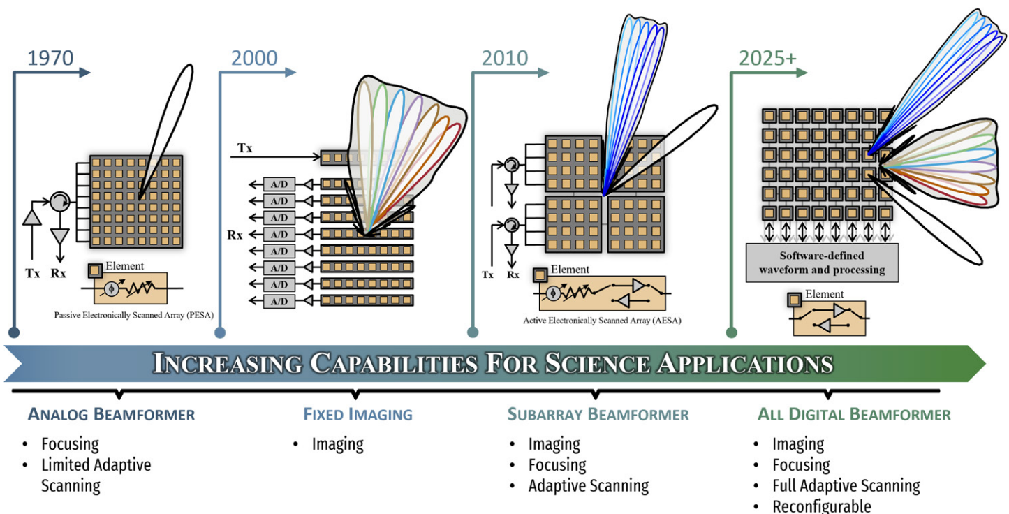
Fig. 6. PAR architectures designed for atmospheric applications: analog beamformer, fixed imaging, subarray beamformer, and all-digital beamformer.
