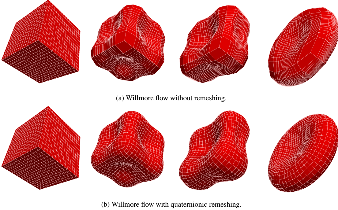
FIGURE 2: Surface area and volume constrained Willmore flow applied to a cube. Here, our remeshing procedure (b) prevents degradation in mesh quality along the flow (a). Note that the minimizing immersion is a biconcave discoid characteristic of biomembranes which are critical for Helfrich-type energies [3, 5]
