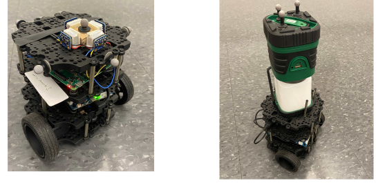
Fig. 10: TurtleBot3 Burger: Left is a mobile sensor with 4 light strength sensors installed on top; Right is the moving light source.
