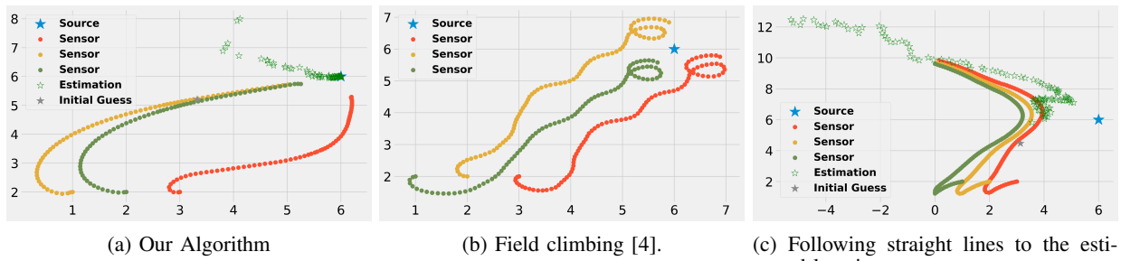
Fig. 3: Comparing the general behavior of seeking a stationary source. The sensors in (b) do not make any estimations, since field climbing only uses measured signal strength to guide sensor movements.
