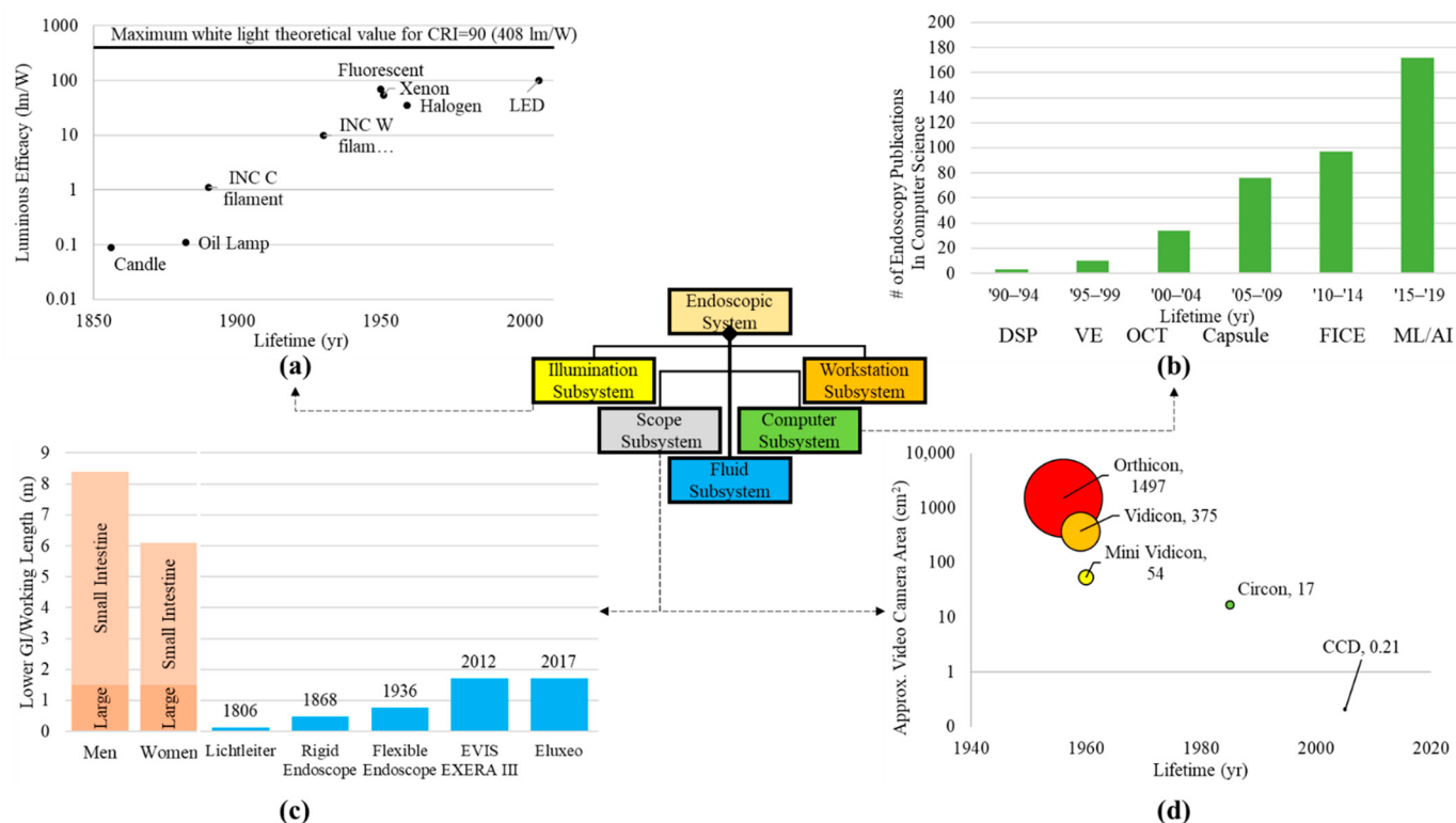
Figure 6. Trends for components within subsystems. (a) Light sources in the illumination subsystem presenting the luminous efficacy from the candle to arc lamps and LEDs. Illumination data were extracted from Azevedo et al.'s paper on solid state lighting [70]. (b) Advancements in computational aspects of endoscope systems were visualized by plotting the increase in endoscopy-related publications within the computer science field (publication search for “endoscopy” in the computer science category per quinquennium—Source: http://www.scopus.com , accessed on 28 July 2022) [75]. Some examples of imaging processing technologies that were found include: digital signal processing (DSP), virtual endoscopy (VE), optical coherence tomography (OCT), capsule endoscopy (Capsule), Fujinon's flexible spectral imaging color enhancement (FICE), and machine learning (ML) [76]. (c) Optical pathway (working length) [22,28,41] for the scope subsystem showing the depth the endoscope has traversed throughout the milestones compared to the length of human body intestinal tract [77]. (d) Approximate camera/detector area for various cameras (both film and digital) throughout imaging in endoscopy. Camera and detector areas were assumed from dimensions given in literature [22,57,78–80].
