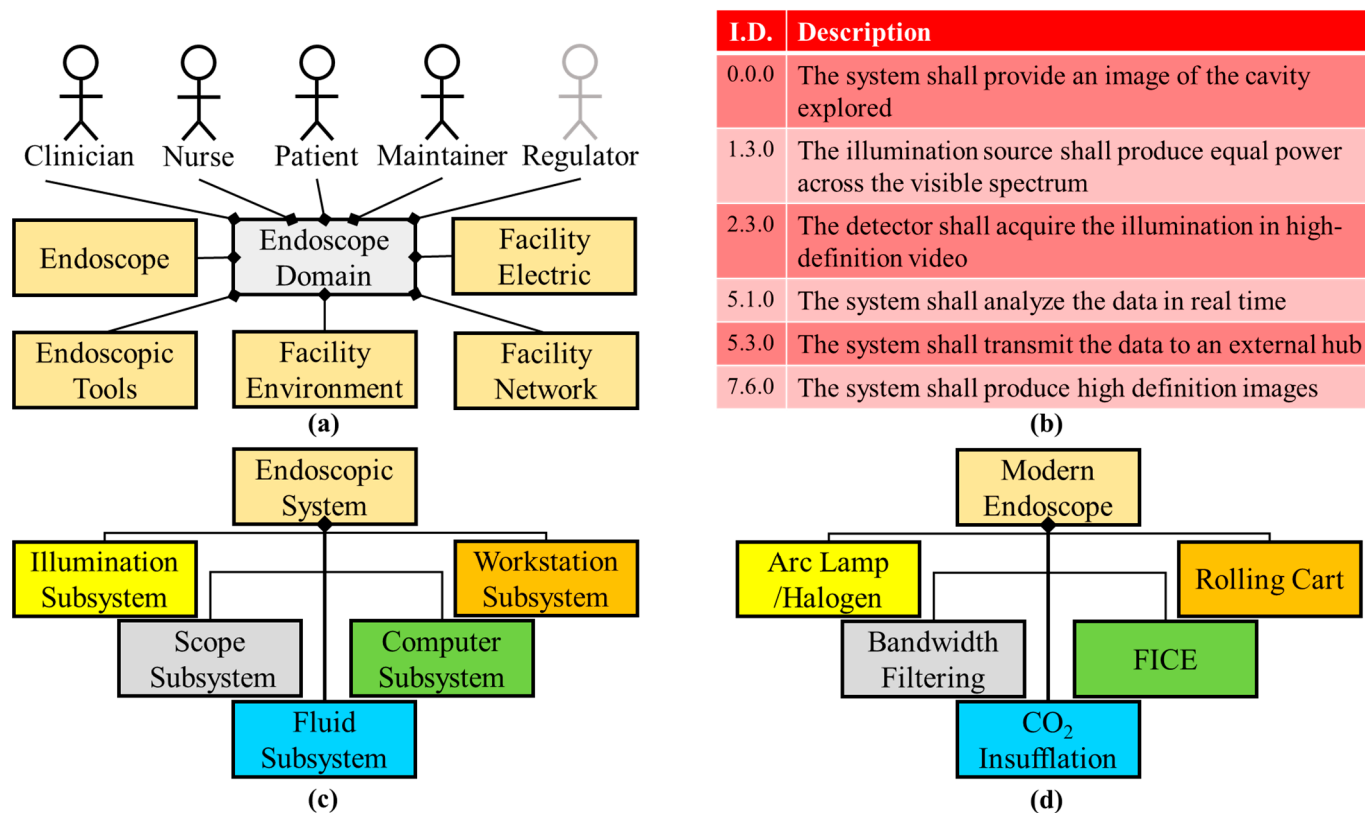
Figure 5. Current endoscope condensed system architecture. (a) The facility network external system was added to the domain diagram of the current system, compared to that of the imaging milestone domain (Figure 4a), because of the use of the internet and cloud storage. (b) High-definition and spectral aspects are stated in the requirements for the current system. (c) The logical diagram remains the same as the previous milestone (Figure 4c). (d) Physical components and software are bandwidth filters and FICE software for this architecture milestone.
