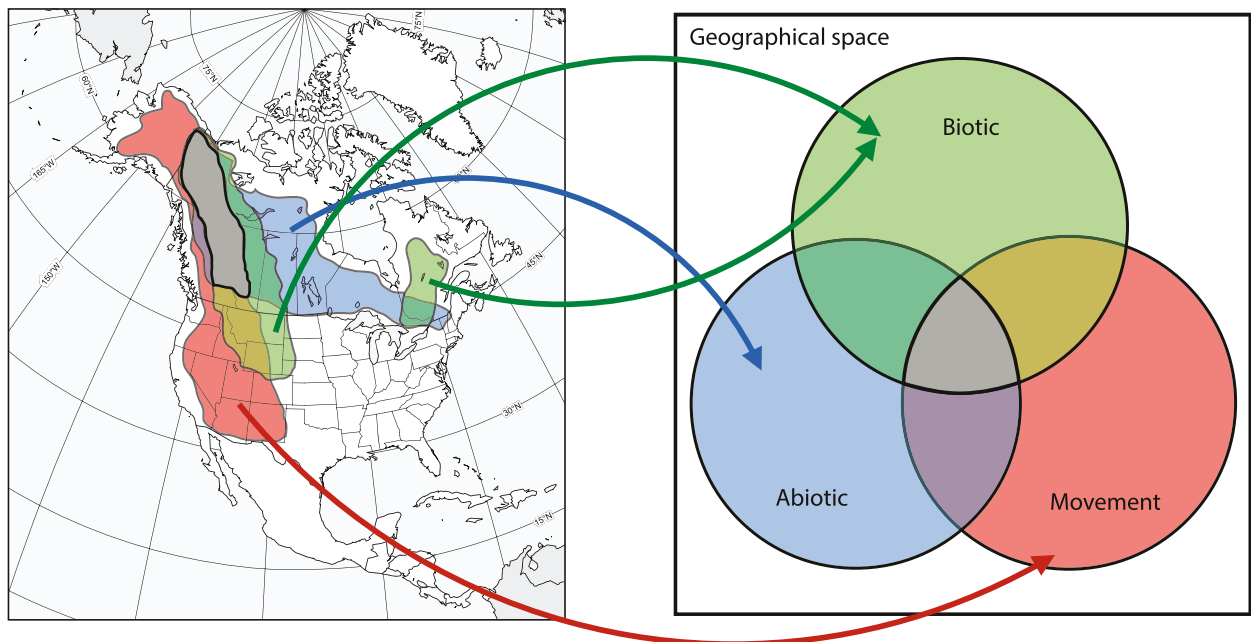
Figure 1: BAM ("biotic, abiotic, and movement") diagram representing the geographical areas where certain ecological and historical conditions required by a hypothetical species are met. The blue area (A) represents the regions in which the abiotic conditions are suitable for the species. The green area (B) represents the regions in which a suitable combination of interacting species occurs. The red area (M) indicates the regions that have been available for a species (e.g., no barriers to dispersal). Areas in the darkest gray match the species' need for all three factors. G represents the total geographical area of the study region. Note that the different sets in the right panel represent a rearrangement of the areas in the map on the left and therefore still represent the extent of suitability in geographical space. Modified from Soberón and Peterson (2005).
