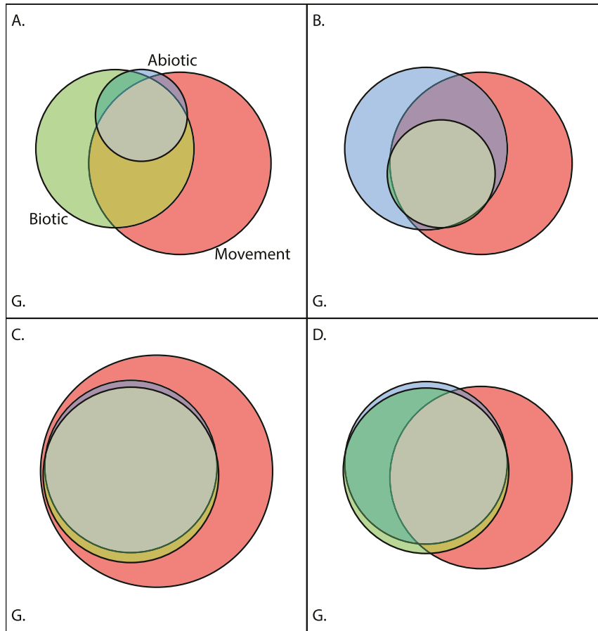
Figure 2: Hypothetical scenarios under which abiotic and biotic factors may limit species distributions represented by different configurations of the BAM ("biotic, abiotic, and movement") diagram. A , Predicted configuration if a species' distribution is limited by abiotic factors. B , Predicted configuration if biotic factors are limiting. C , Predicted distribution if both of these factors limit the species' distribution. D , Predicted configuration if "movement" restrictions or other factors not captured by the biotic or abiotic variables are limiting, beyond the confounded effects of abiotic and biotic factors. The lower panels represent configurations in which biotically and abiotically suitable areas are congruent.
