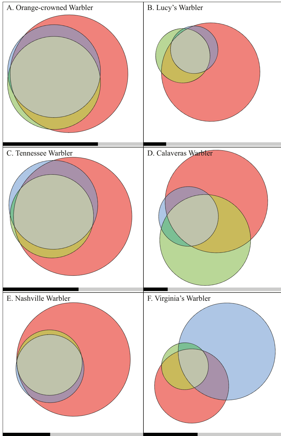
Figure 5: Empirical BAM (“biotic, abiotic, and movement”) diagrams calculated for each species of warbler examined in this study. Blue areas represent abiotically suitable regions based on climate-only ecological niche models (ENMs). Green areas represent biotically suitable regions based on pollen-only ENMs. Red areas represent available areas within which movement-related factors are not expected to be limiting (see text). The length of the black bar at the bottom of each diagram is proportional to the total area of the union of A, B, and M, indicating the “zoom” for each species relative to the whole of North America (the sum of the black bar and the gray bar).
