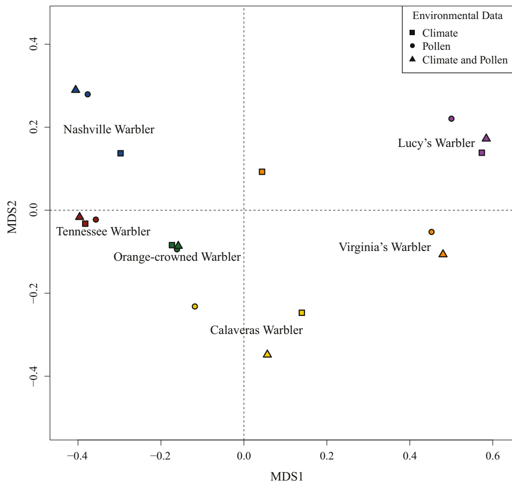
Figure 4: Multidimensional scaling plot showing the relationship among the projected suitable areas for all species of warblers examined in this study. This plot visualizes the overall distances ( 1 - \text{Schoener's } D ) between climate-only ecological niche models (ENMs; squares), pollen-only ENMs (circles), and climate-and-pollen ENMs (triangles) for each species (different colors).
