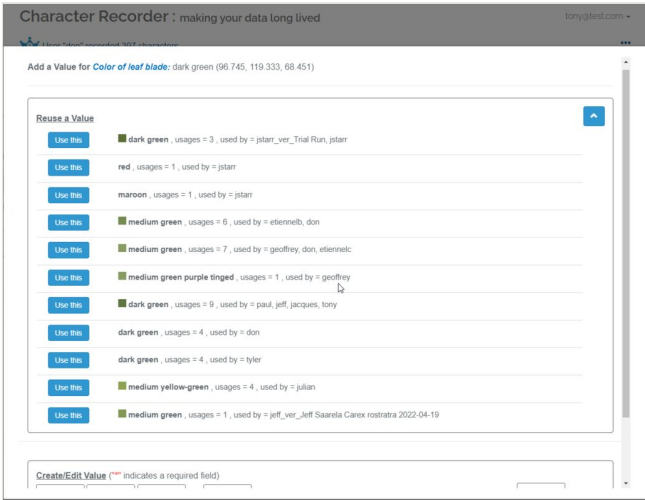
Figure 4. Variation in recorded values for Color of leaf blade . Some users picked colors from Character Recorder's color palettes, while others chose to enter string values.
