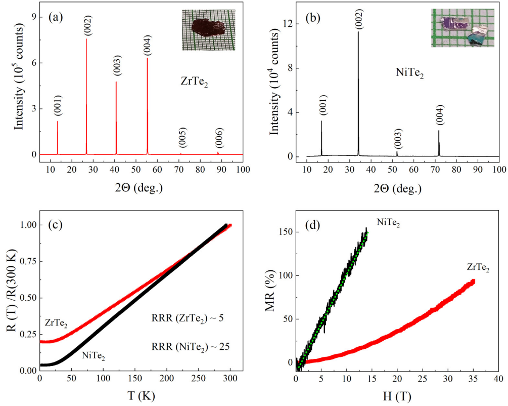
FIG. 1. XRD, electrical resistance, and MR. Room-temperature XRD pattern of (a) \text{ZrTe}_2 and (b) \text{NiTe}_2 single crystals indexed in P\bar{3}m1 structures. Insets in (a) and (b) show typical single crystals of \text{ZrTe}_2 and \text{NiTe}_2 , which are 8 \times 8 \times 0.2 and 3 \times 2 \times 0.3 mm 3 , respectively. (c) R vs T graph for \text{ZrTe}_2 and \text{NiTe}_2 . R(T) is normalized with the room-temperature value. Resistance for both samples decreases with T , showing a typical metallic behavior. (d) MR of \text{ZrTe}_2 and \text{NiTe}_2 samples up to 35 and 14 T, respectively. \text{NiTe}_2 shows a linear MR, whereas \text{ZrTe}_2 has a parabolic dependence on the applied field. There is no signature of SdH oscillations in MR for either sample. The dashed line is a guide to an eye.
