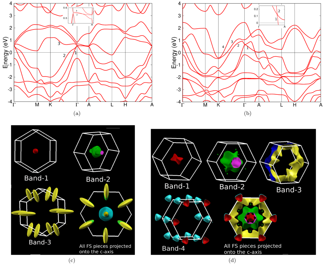
FIG. 4. Electronic band structure and Fermi surface. Band structure and Fermi surface of (a) and (c) ZrTe 2 and (b) and (d) NiTe 2 calculated with the inclusion of spin-orbit coupling. The insets in (a) and (b) show zoomed-in bands in a small energy window above the Fermi level to highlight the type-II Dirac crossings along the \Gamma -A direction. In order to identify the bands which cross the Fermi surface, we have labeled the bands based on their energy. See text for details.
