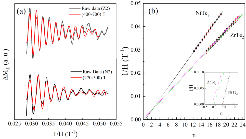
FIG. 3. The bandpass filter and LL fan diagram. (a) The dHvA oscillations for ZrTe 2 at \theta = -20^\circ and NiTe 2 at \theta = 20^\circ . Bandpass filters of 400–700 and 270–500 T are used to select oscillations corresponding to F_\alpha and \bar{F}_\beta . The black and red curves represent the raw data and filtered data, respectively. (b) The LL fan diagram for ZrTe 2 ( F_\alpha ) and NiTe 2 ( \bar{F}_\beta ). Minima and maxima of the oscillations are assigned to (n - 1/4) and (n + 1/4) , respectively, to construct the LL plot. The error bar for each data point is taken as the half-width at half maximum of the respective peak position. The dashed lines are the linear extrapolations of the data. The inset shows the LL plot in the limit 1/H \rightarrow 0 .
