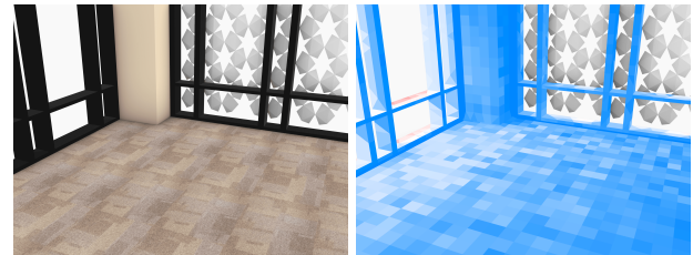
Figure 6: (Left) An example BIM data visualization of our test building environment with a facade design in place. (Right) An example daylighting radiation analysis applied. The BIM data is matched in reality to visualize the designs and daylighting in AR.
