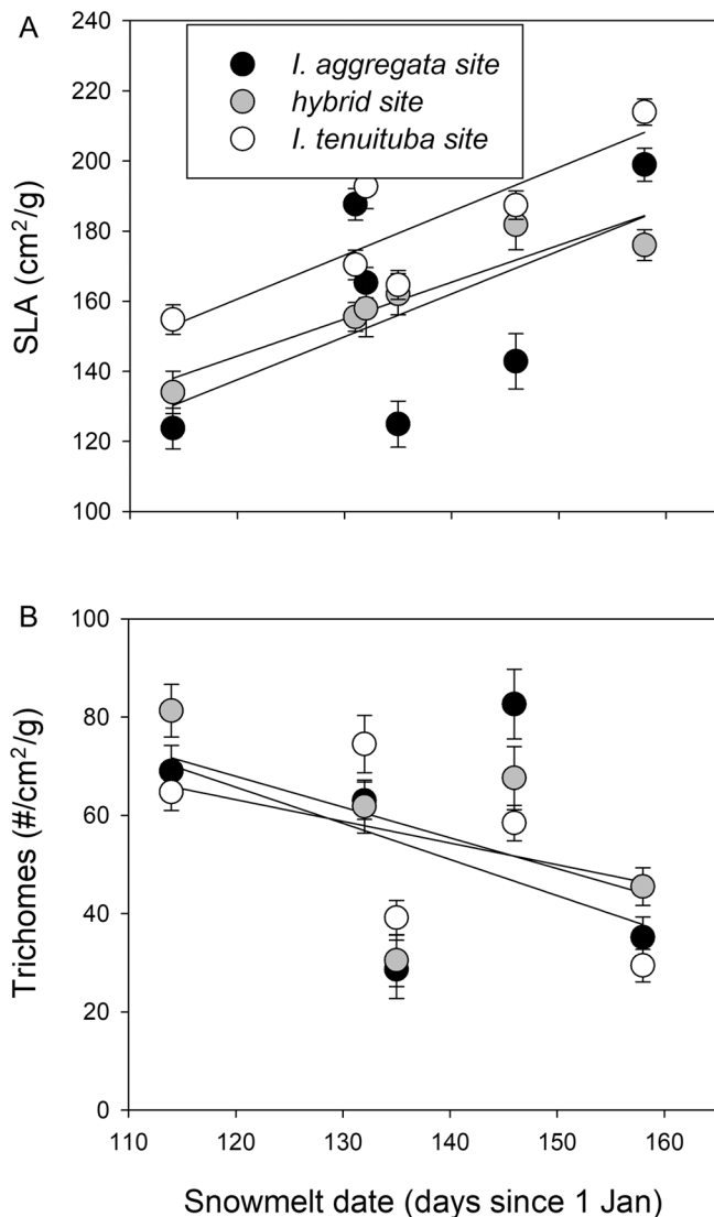
FIGURE 2 Changes in (A) specific leaf area (SLA) and (B) trichome density with snowmelt date for Ipomopsis plants. Values plotted are least squares means and SE from repeated measures analysis.
