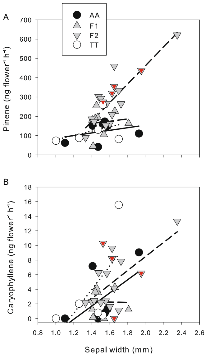
FIGURE 3 Family mean values for (A) pinene and (B) \beta -caryophyllene plotted against sepal width. Regression lines are fit separately for each source (AA, F 1 , F 2 , TT). AA = Ipomopsis aggregata \times I. aggregata . TT = I. tenuituba \times I. tenuituba . F 1 and F 2 are hybrids. Slopes differed significantly from zero for pinene in the F 2 ( P < 0.0001 ) and caryophyllene in F 2 and TT ( P = 0.0108 and 0.0148 ). The four outbred F 2 families are indicated by red symbols.
