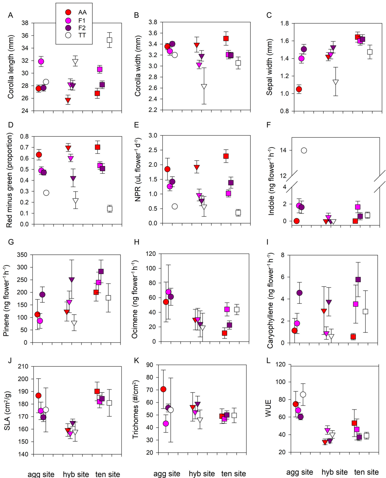
FIGURE 1 Trait means and standard errors for four source types (AA, F 1 , F 2 , TT) planted as seeds at three sites ( Ipomopsis aggregata , hybrid, I. tenuituba ). AA = I. aggregata × I. aggregata . TT = I. tenuituba × I. tenuituba . F 1 and F 2 are hybrids. (A–C) Floral morphometric traits. (D) Petal color. (E) Nectar production. (F–I) Floral volatiles. (F) The one I. tenuituba plant measured for indole at the I. aggregata site had an unusually high value, but similarly high values have been seen for other I. tenuituba individuals (Campbell et al., 2022a). (J–L) Vegetative traits.
