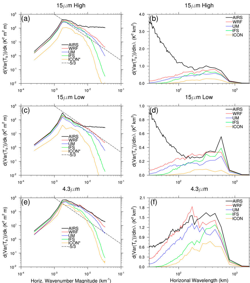
FIG. 7. The sum of brightness temperature perturbation spectra for all overpasses plotted on (left) log–log axis and (right) linear–log axis. Areas under the curves in the right column are proportional to area-integrated T'_b in each overpass in Fig. 3 and further summed over all overpasses (i.e., \propto \sum_{N_{op}} \text{Var}(T'_b) , where \text{Var}(T'_b) = \iint T'_b dx dy and N_{op} is the number of overpasses). Results from the (top) 15- \mu\text{m} high ( z \approx 41 km), (middle) 15- \mu\text{m} low ( z \approx 24 km), and (bottom) 4.3- \mu\text{m} ( z \approx 37 km) products are shown.
