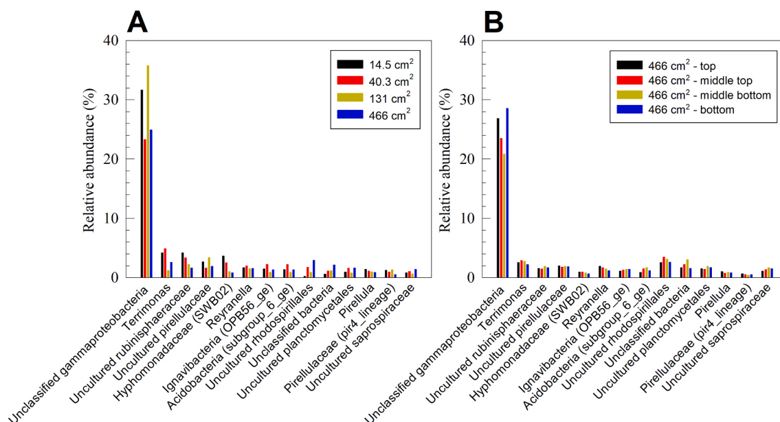
Fig. 5. Genus-level 16 S rRNA gene microbial community analysis of A) four oxygen-reducing cathodic biofilms (surface areas = 14.5 cm 2 , 40.3 cm 2 , 131 cm 2 and 466 cm 2 ), and B) 466 cm 2 cathodic biofilm sampled at four different locations. The data show that the microbial community structure is independent of cathode size, and of the location within the cathode.
