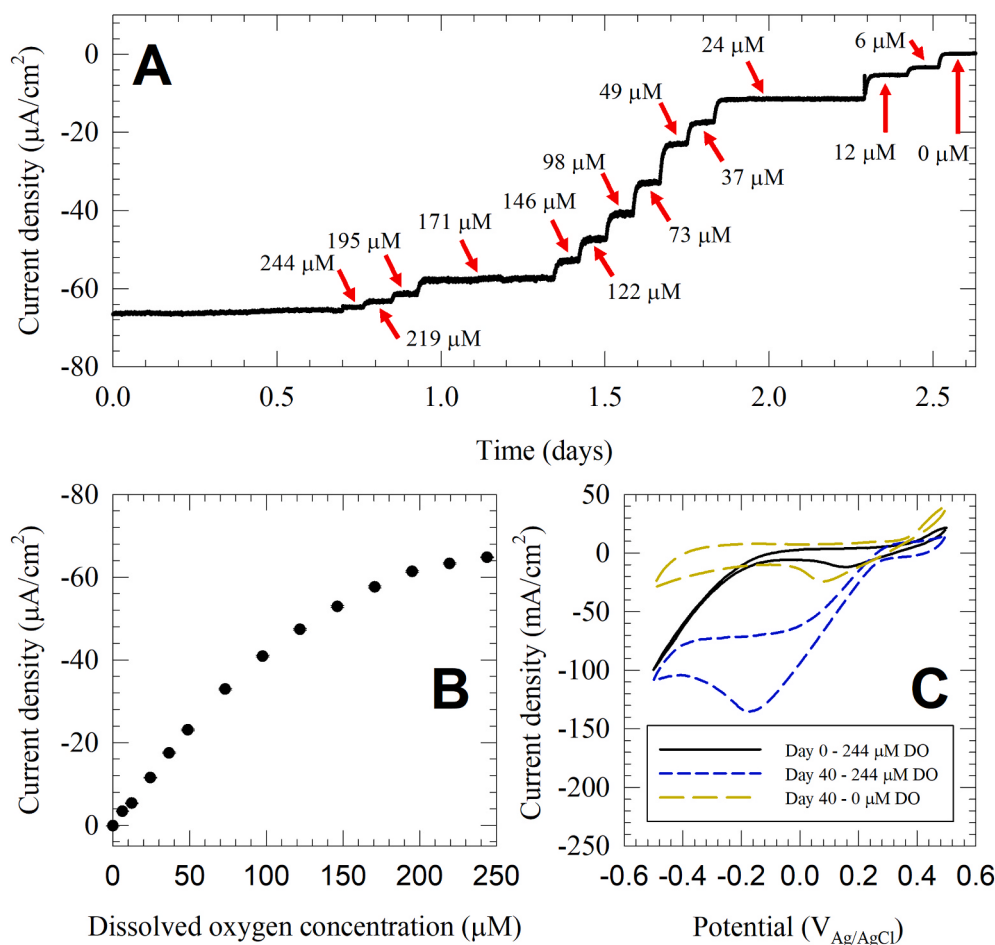
Fig. 1. An example dataset showing current changes as response to change in bulk DO concentration for a biofilm enriched on a 131 \text{cm}^2 electrode catalyzing oxygen reduction reaction. A) The response of the cathodic biofilms to change in DO concentration from 244 \mu\text{M} –0 \mu\text{M} . B) The dependency of cathodic current on DO concentration. C) Cyclic voltammograms of the abiotic control (day 0, 244 \mu\text{M} DO concentration), enriched cathodic biofilm in the presence and absence of oxygen (day 40, 244 \mu\text{M} and 0 \mu\text{M} DO concentration, respectively).
