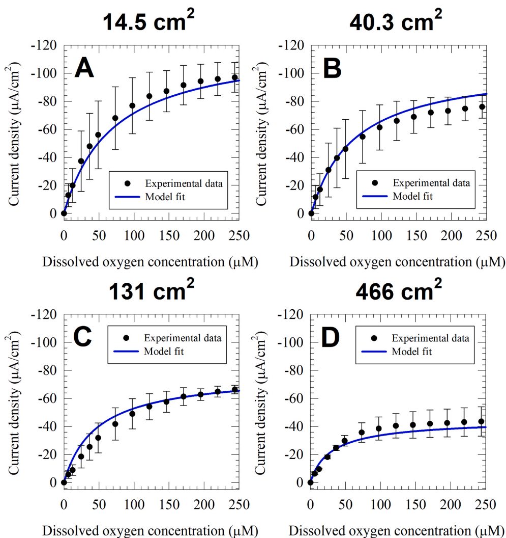
Fig. 2. Experimental and model best-fit current of oxygen reducing cathodic biofilms in response to change in DO concentration from 244 \mu\text{M} to 0 \mu\text{M} , A) 14.5 \text{cm}^2 , B) 40.3 \text{cm}^2 , C) 131 \text{cm}^2 , and D) 466 \text{cm}^2 . The data represent the average of three biological replicates, and the error bars represent the standard deviation.
