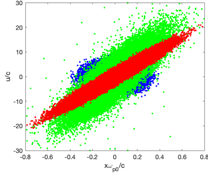
FIG. 2: Phase space coordinates of 100,000 particles for an initial beam matrix shown in blue. Red indicates particle coordinates having propagated through a transfer matrix and green show the coordinates for the corresponding nonlinear matrix with randomly sampled \delta\gamma .
