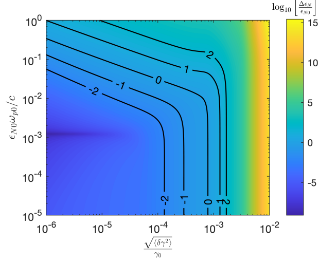
FIG. 7: Relative emittance growth \Delta\epsilon_N/\epsilon_{N0} through 85 accelerating stages as a function of initial relative energy spread \sqrt{\langle\delta\gamma^2\rangle}/\gamma_0 and initial normalized emittance \epsilon_{N0} . The colormap / contours show the base-10 logarithm of \Delta\epsilon_N/\epsilon_{N0} .
