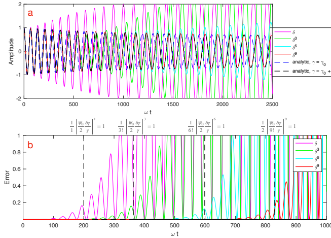
FIG. 9: Betatron oscillations modelled using the expanded nonlinear transfer matrix in Eqn. (B4). (a) Oscillations with an increasing \gamma factor from \gamma_0 = 100 to \gamma_0 = 500 corresponding to linear acceleration. The dashed lines correspond to analytic (WKB) solutions for betatron oscillations for the design \gamma = \gamma_0 (blue) and \gamma = \gamma_0 + \delta\gamma (black), for a energy deviation \delta\gamma = 10 . The colored solid lines indicate solutions using the nonlinear matrix with different orders in \delta = \delta\gamma/\gamma up to the \delta^9 th term, i.e. m = 9 . (b) The error in the solution for oscillations with fixed \gamma = 100 , defined as |x_{n\delta m} - x|^2 , where x is the analytic solution and x_{n\delta m} is the matrix solution including terms up to m . The black dashed lines show the thresholds |\frac{\psi_0 \delta\gamma}{2\gamma}|^m / m! = 1 corresponding to Eqn. (B5).
