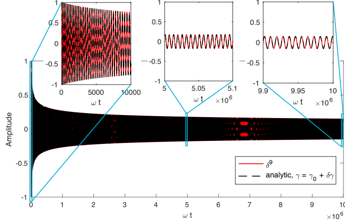
FIG. 10: Demonstration of method accuracy; Betatron oscillations for particle linearly accelerated with design energy \gamma = 1000 to 2 \times 10^6 over a total time of \omega t = 10^7 , where the betatron frequency is \omega/\sqrt{\gamma} , with a deviation from the design energy of \delta\gamma = 20 , i.e. corresponding to an initial relative energy spread \delta\gamma/\gamma = 2\% . The main panel shows the (unresolvable) oscillations for a WKB solution compared with the nonlinear matrix solution including terms up to m = 9 over the full range. The inset panels show expanded regions at the beginning, middle and end.
