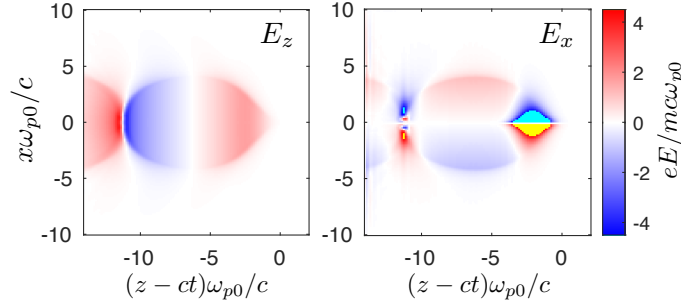
FIG. 4: Fields taken from the 3D simulation at \omega_{p0}t = 9000 in the z - x plane at y = 0 . (left) Accelerating ( E_z ) field and (right) focusing ( E_x ) field.
