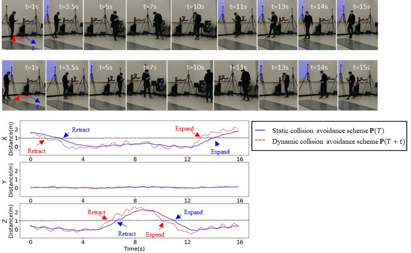
Figure 4. Preliminary validation of the proposed collision avoidance schemes. Top: A robot operator approached the co-robot in x-direction, turned right, and left in z-direction. This operator then turned back, approached the robot in -z -direction, turned left, and left the co-robot in x-direction. The first row of the key frames shows the co-robot's behavior when static collision avoidance scheme is adopted. The second row shows the co-robot's behavior when dynamic collision avoidance scheme is adopted. Bottom: The P(T) in the static collision avoidance scheme and P(T + t) in dynamic collision avoidance scheme are compared over time. The two curves are matched by the initial time instant of operator's move. Co-robot arm retraction and expansion time instants are marked. The co-robot responds earlier to the worker's approaching/leaving motion when dynamic collision avoidance scheme is applied.
