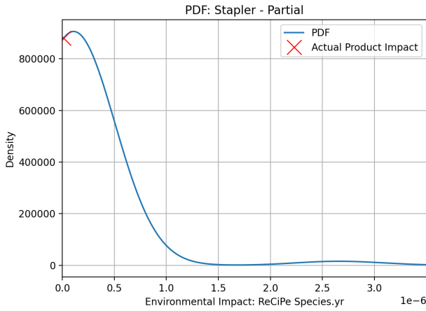
(c) Stapler partial BOM probability density function
