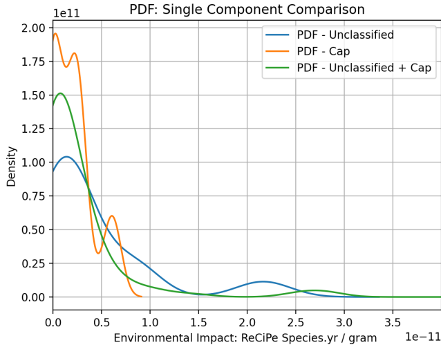
FIGURE 7: Probability density function for Cap, Unclassified and Cap + Unclassified component(s)
