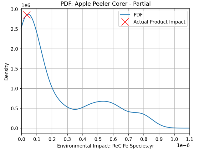
(b) Apple Peeler Corer partial BOM probability density function
