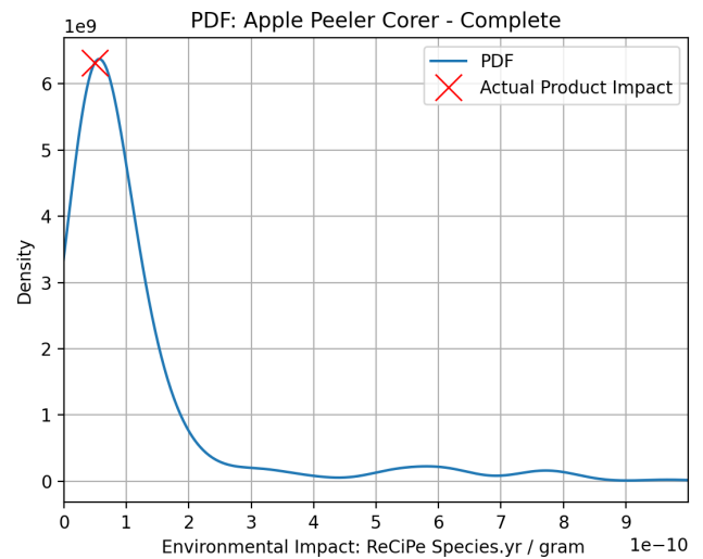
FIGURE 3: Probability density function for the complete Apple Peeler Corer bill of materials
