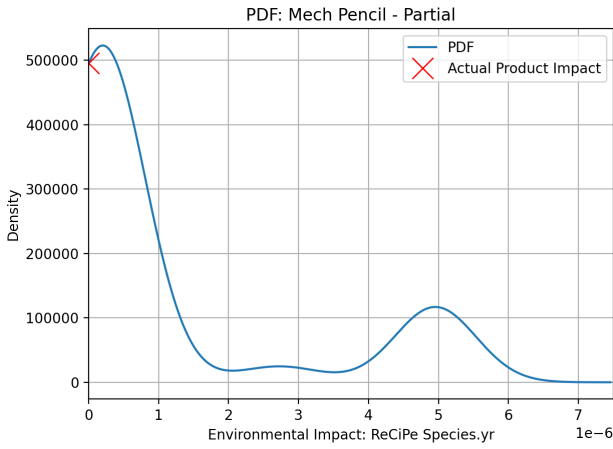
(a) Mechanical Pencil partial BOM probability density function
