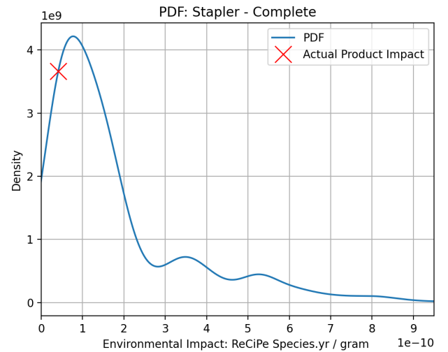
FIGURE 4: Probability density function for the complete Stapler bill of materials
