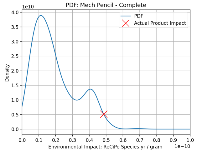
FIGURE 2: Probability density function for the complete Mechanical Pencil bill of materials
