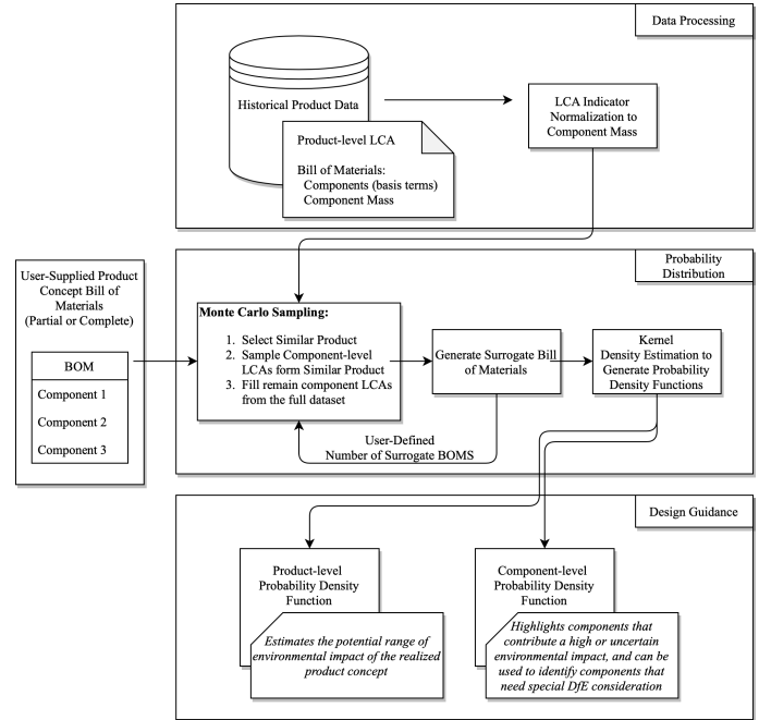
FIGURE 1: PeeP method overview
