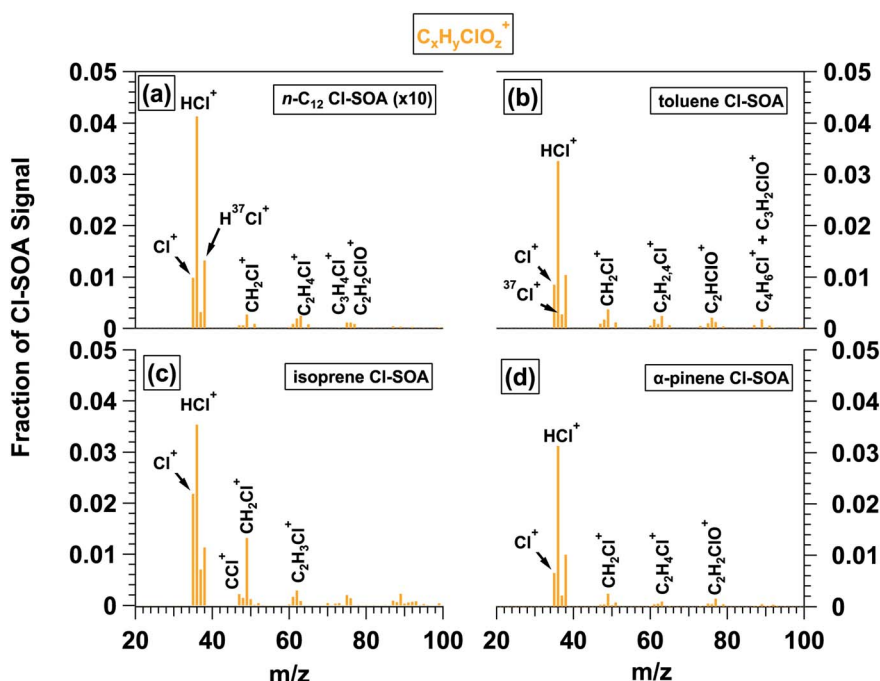
Fig. 3 \text{C}_x\text{H}_y\text{ClO}_z^+ ions present in L-ToF-AMS spectra of (a) n\text{-C}_{12} , (b) toluene, (c) isoprene, and (d) \alpha -pinene Cl-SOA displayed in Fig. 1b, d and 2b, e. The y-axis scale in (a) is multiplied by 10 to put it on the same scale as (b)–(d).
