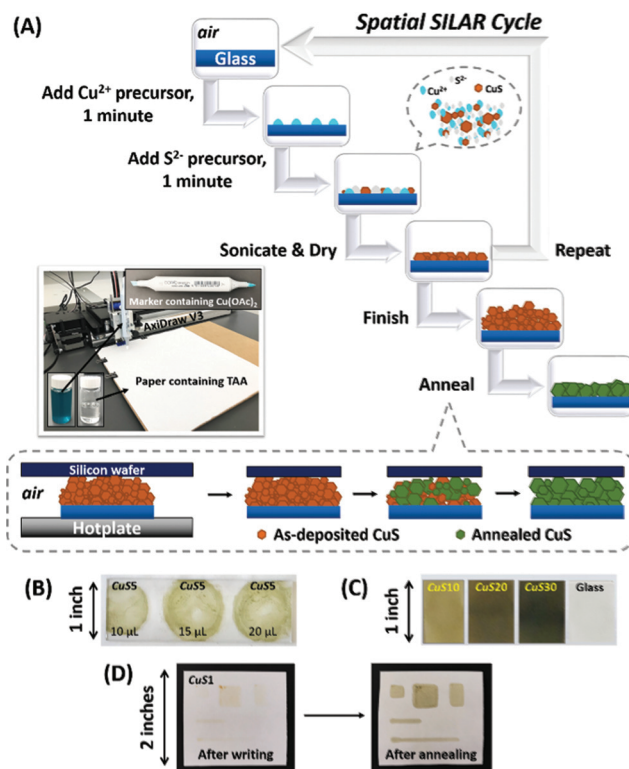
Scheme 1 (A) Schematics of the Spatial SILAR with low-temperature post-annealing. The insets are optical photos of a lab-designed automatic thin-film fabrication system by AxiDraw V3 and the precursor solutions for CuS. All materials in the schematics are not in real scale/ratio. Optical photos of: (B) a series of CuS 5 prepared on an untreated glass slide as a control, (C) CuS 10-30 prepared on SC-1-treated glass slides for SEIRA study and a blank glass substrate as reference, and (D) different patterns of CuS 1 written on a piece of standard US letter paper by AxiDraw V3.
