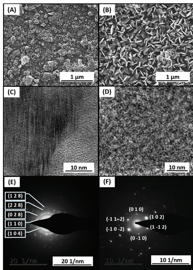
Fig. 1 (A and B) SEM and (C and D) TEM images of as-deposited and annealed CuS thin films, respectively, and (E and F) the corresponding SAED patterns.
