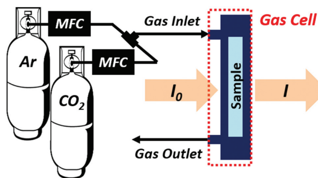
Scheme 2 Schematics of the gas sensing setup. MFC: mass flow controller; I_0 : incident light; I : emergent light. All materials are not in real scale/ratio.
