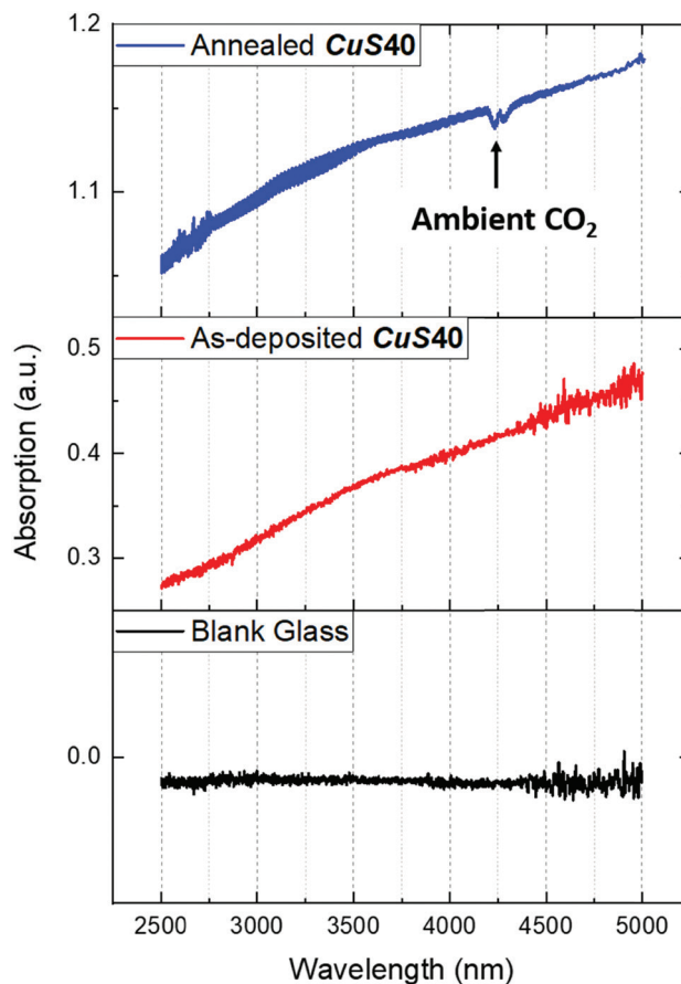
Fig. 2 FTIR ATR absorption spectra of as-deposited and annealed CuS40, and a blank glass substrate measured under standard ambient conditions.
