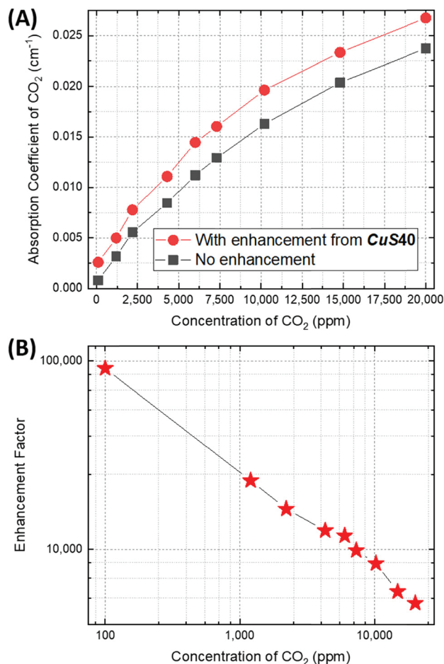
Fig. 3 (A) Experimental IR absorption coefficient of CO 2 (at approximately 2683 cm -1 ) as a function of concentration, obtained with/without the enhancement from CuS40 . (B) Calculated IR absorption enhancement factor for CO 2 provided by CuS40 .
