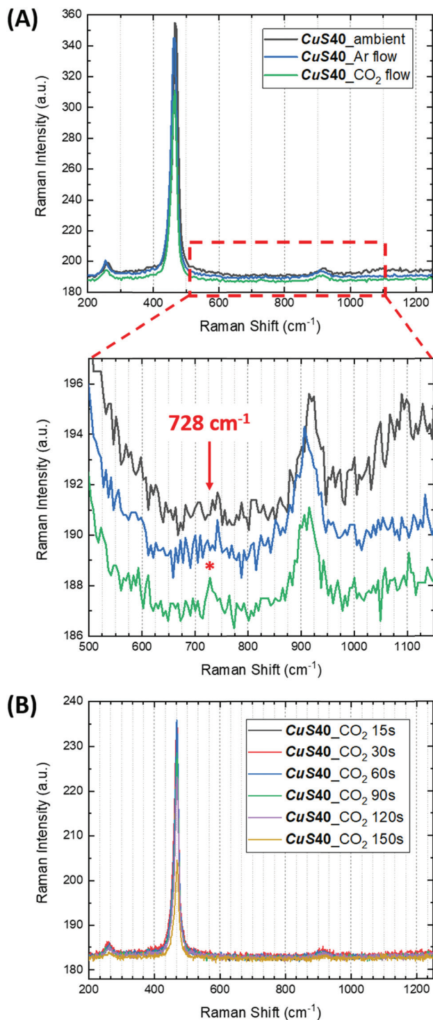
Fig. 4 (A) Raman spectra of annealed CuS40 collected under standard ambient conditions, and the in situ measurement while flowing Ar (100.00%) and CO 2 (100.00%), respectively, and a magnified view of the selected area indicated by the red dashed line. (B) In situ Raman spectra of annealed CuS40 collected after exposing to a flow of CO 2 for different time (in seconds).
