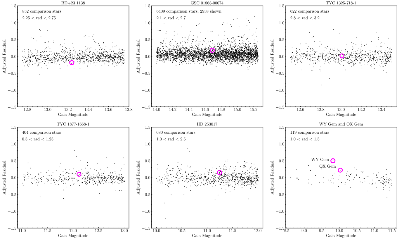
Figure 13. Stars 1, 2, 3, 5, 7, and a combination of 4 and 8 respectively (see Table 3). The magenta circles identify the star in question. The y-axis is the residual after removing the trend with pg and adjusting the mean to be zero. Thus the y-value of the magenta circle is the offset indicated in Table 3
