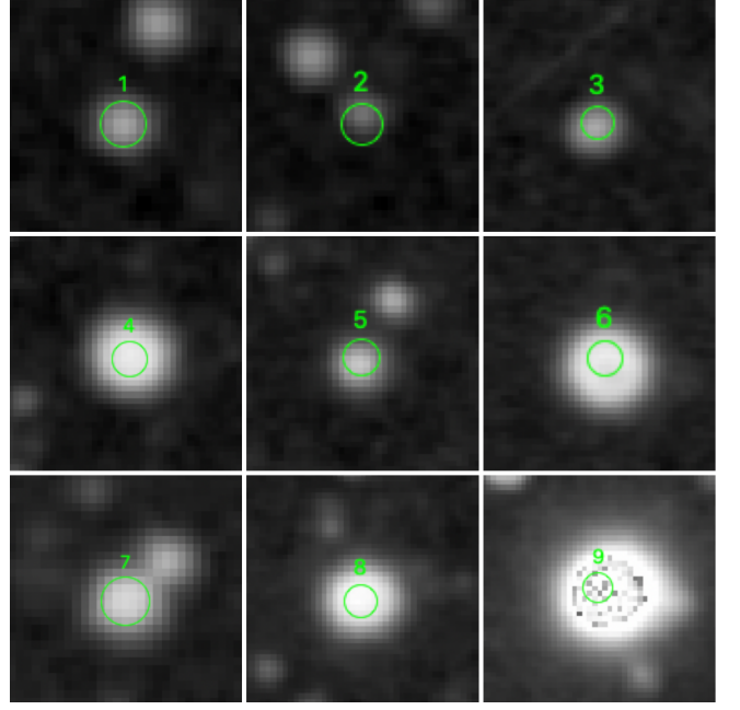
Figure 12. Cut-out images of the stars in common with the MB19 catalog of red supergiants, ordered by increasing R.A. The green circle is the 3-pixel-radius measurement aperture. Star 9 ( \eta Gem) shows the effect of central values exceeding the 16-bit limit.
