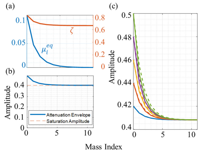
FIG. 4. Perturbation results for transitional evanescent waves. (a) The evolution of the local decay factor \zeta and the equivalent imaginary wave-number component \mu_i^{\text{eq}} in the downstream direction. (b) The nonlinear attenuation envelope and the saturation amplitude. (c) Attenuation envelopes initiated at varying amplitudes. The solid and dashed curves represent envelopes obtained from a spatially varying \zeta and a uniform exponential index \zeta^* computed from the convergence, respectively.
