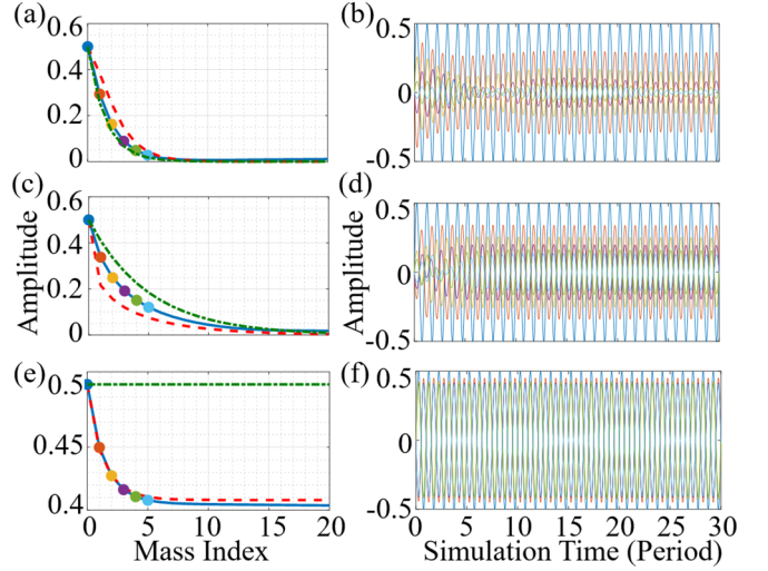
FIG. 5. Numerical verification of complete and transitional evanescent waves for initial-condition excitation. (a), (c), and (e) Comparison between perturbation-predicted (red dashed line), numerically simulated (blue solid line), and linear (green dash-dotted line) amplitude envelopes for hardening nonlinearity ( \bar{\omega} = 2.1 ), softening nonlinearity ( \bar{\omega} = 2.01 ), and softening nonlinearity ( \bar{\omega} = 1.95 ) with saturation effect. The numerical time responses of the first five masses in the system are plotted on the right in panels (b), (d), and (f). The color of each curve in panels (b), (d), and (f) is associated with the color of the mass identified on the left.
