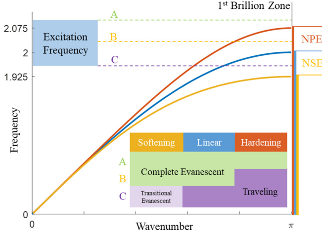
FIG. 2. Nonlinearly shifted dispersion for propagating waves (i.e., real wave numbers) in a monatomic chain, with amplitude |A| = 0.5 . Blue, red, and yellow curves represent the linear, hardening, and softening nonlinear dispersions, respectively. The corresponding cutoff frequencies are marked on the vertical axis. The nonlinear passband extension (NPE) and nonlinear stopband extension (NSE) are indicated to the right. Three example signal frequencies and their corresponding wave forms in each system are presented in the embedded table.
