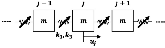
FIG. 1. The schematic of the studied nonlinear monatomic system.
