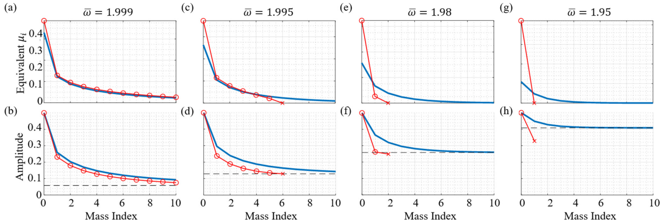
FIG. 7. The saturation effect derived from standard and modified perturbation results. Each column features the resultant imaginary wave-number component (top row) and attenuation envelope (bottom row) for selected frequencies. In each subfigure, blue solid curves denote the result from the modified perturbation result, and red solid curves denote the standard perturbation result. A round marker refers to a valid result, and a cross marker suggests an invalid one since the amplitude at this point is below the saturation amplitude indicated by the gray dashed line.
