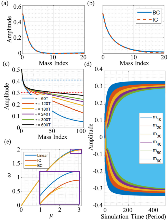
FIG. 6. Numerical verification with boundary-continuous excitation. (a) Numerical attenuation envelopes of a complete evanescent wave in a hardening system resulting from BC and IC excitation. (b) The numerical attenuation envelopes of a complete evanescent wave in a softening system resulting from BC and IC excitation. (c) The numerical attenuation envelope with selected simulation time (measured in excitation period T ) for amplitude A = 0.5 . The blue and red dashed lines indicate the saturation amplitude predicted from initial-condition excitation and boundary-continuous excitation, respectively. (d) Time responses of selected masses for A = 0.5 . (e) Band-clipping effect on the studied system for A = 0.3 . The green dashed line in the zoomed-in view denotes the excitation frequency.
