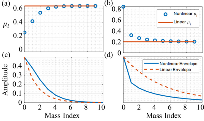
FIG. 3. Results for nonlinear and linear complete evanescent waves. The top row depicts the evolution of the imaginary wave number along the downstream direction, while the bottom row translates the imaginary wave number into a discrete attenuation envelope; the left column corresponds to a hardening nonlinear system, and the right column corresponds to a softening system.
