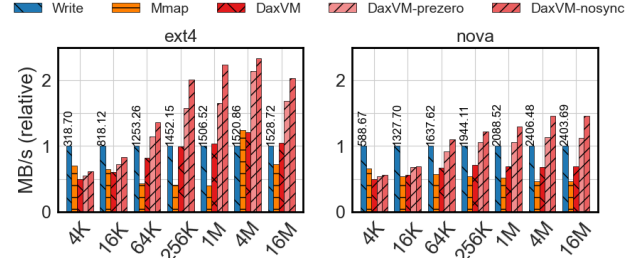
Figure 7: Append operations.
