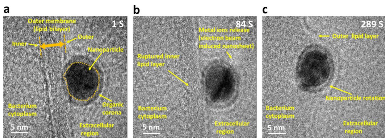
Figure 1. In-situ graphene liquid cell HR-TEM micrographs representing the event dynamics of (Fe/Ni/Cu) ternary nanoparticle internalization pathway by Escherichia Coli bacterial cell membrane. (a) HR-TEM micrograph indicating the outer bacterial cell membrane (lipid bilayer) and a nanoparticle with organic corona attached with the bacterial cell membrane. (b) HR-TEM micrograph confirming the ruptured inner lipid layer and split outer lipid layer during the event of nanoparticle internalization. (c) HR-TEM micrograph confirming the complete internalization of nanoparticle by bacterial cell with the surrounding outer lipid layer.
