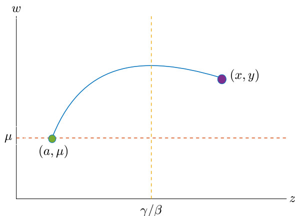
Fig. 2. Graph of w = (\gamma/\beta) \ln z - z + \psi(x, y) for a \leq z \leq x . Here x > 0 , y > \mu , and a = a(x, y) \in (0, \gamma/\beta] is the unique solution of \psi(x, y) = \psi(a, \mu) .
