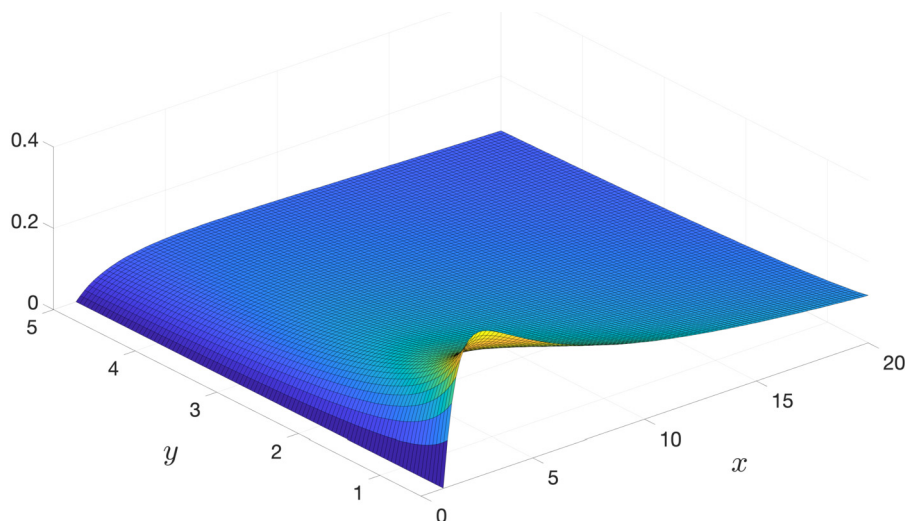
Fig. 5. Numerical approximation of the function v(x, y) for (x, y) \in [1, 20] \times [1/2, 5] . Here \beta = \gamma = 3 . Consult the appendix for an explanation of how we arrived at this graph.
