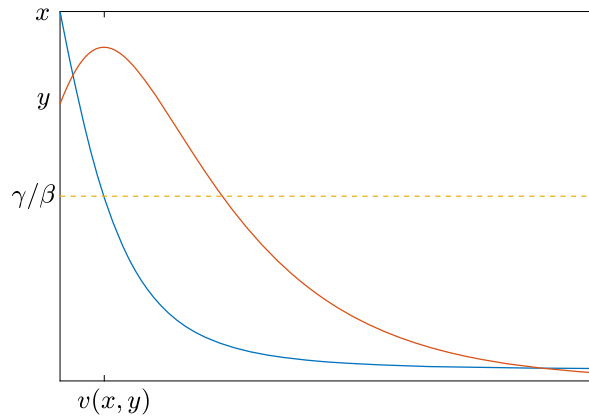
Fig. 3. The solution pair S, I of (1.1) with S(0) = x and I(0) = y . S(t) is shown in blue and I(t) is shown in red. Note that v(x, y) is the first time S(t) \leq \gamma/\beta which is also the same time that I starts to decrease.
