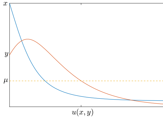
Fig. 1. Plot of the solution pair S, I of (1.1) with S(0) = x and I(0) = y . S(t) is shown in blue and I(t) is shown in red. Note that u(x, y) is the first time t such that I(t) \leq \mu . (For interpretation of the colors in the figure(s), the reader is referred to the web version of this article.)
