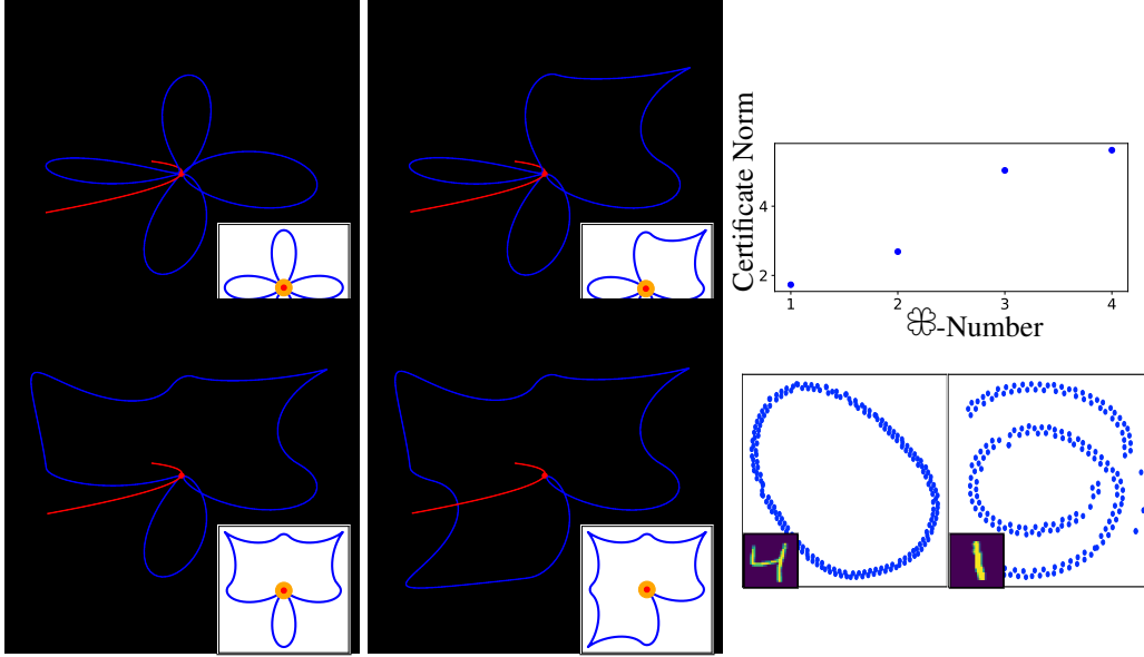
Figure 2: The \text{clover} -number—theory and practice. Left: We generate a parametric family of space curves with fixed maximum curvature and length, but decreasing \text{clover} -number, by reflecting ‘petals’ of a clover about a circumscribing square. We set \mathcal{M}_+ to be a fixed circle with large radius that crosses the center of the configurations, then rescale and project the entire geometry onto the sphere to create a two curve problem instance. In the insets, we show a two-dimensional projection of each of the blue \mathcal{M}_- curves as well as a base point \mathbf{x} \in \mathcal{M}_+ at the center (also highlighted in the three-dimensional plots). The intersection of \mathcal{M}_- with the neighborhood of \mathbf{x} denoted in orange represents the set whose covering number gives the \text{clover} -number of the configuration (see (2.2)). Top right: We numerically generate a certificate for each of the four geometries at left and plot its norm as a function of \text{clover} -number. The trend demonstrates that increasing \text{clover} -number correlates with increasing classification difficulty, measured through the certificate problem: this is in line with the intuition we have discussed. Bottom right: t-SNE projection of MNIST images (top: a “four” digit; bottom: a “one” digit) subject to rotations. Due to the approximate symmetry of the one digit under rotation by an angle \pi , the projection appears to nearly intersect itself. This may lead to a higher \text{clover} -number compared to the embedding of the less-symmetric four digit. For experimental details for all panels, see Appendix A.
