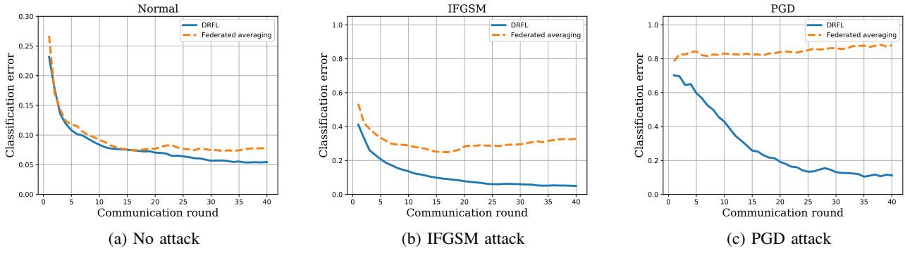
Fig. 1: Federated learning for image classification using the MNIST dataset.
