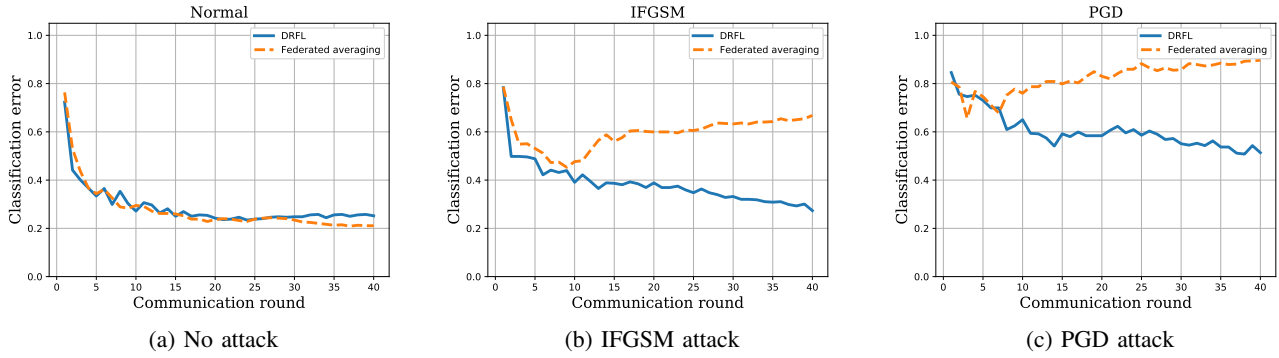
Fig. 2: Distributionally robust federated learning for image classification using F-MNIST dataset.
