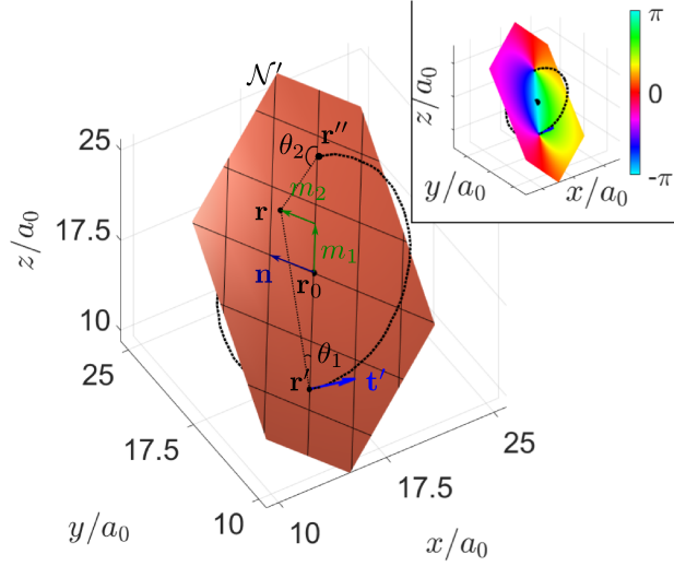
Figure A.7: Geometry of the circular dislocation loop in a slip plane given by the normal vector \mathbf{n} . \mathcal{N}' is the plane normal to the tangent vector \mathbf{t}' upon which we impose a Cartesian coordinate system to determine the angles \theta_1, \theta_2 that are used to construct the (inset) initial amplitude phase configuration. For more details, see Section Appendix A.4.
