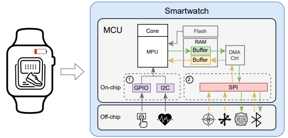
Fig. 1: Architecture of an MCU-based smart watch. ① Slow MMIO-based data flows, ② Real-time and high-throughput DMA-based data flows.
