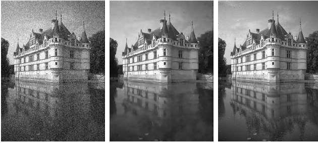
Figure 1: Left: Noisy image f with \sigma = 25 ; Middle: solution of (7), TNRD(f) , with u(t=0) = f , PSNR=29.64, SSIM=0.8496, Right: solution of (5) with \lambda = 0 , an oracle \kappa_F = \kappa(a) and f_{in} = TNRD(f) , PSNR=33.69, SSIM=0.9289.
