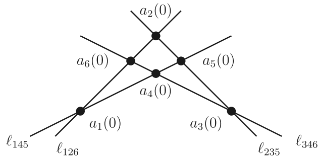
Fig. 20. Degeneration of six points in \mathbb{P}^2 .
