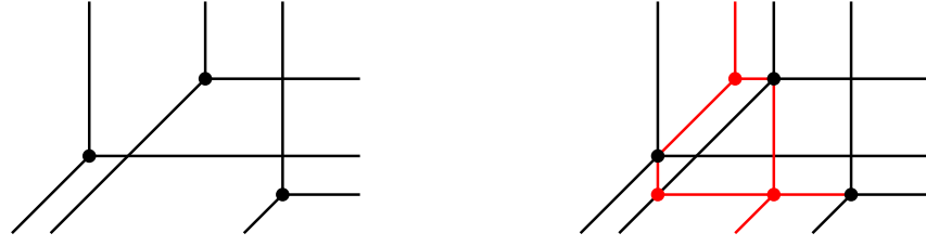
Fig. 16. Example of \mathcal{S}(v) (on the left) and its refinement \tilde{\mathcal{S}}(v) (on the right).
