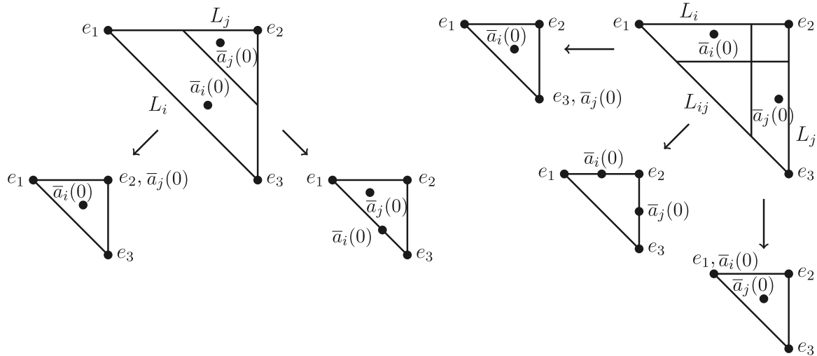
Fig. 15. In the proof of Lemma 9.2, the central fibers of the Mustafin joins \mathbb{P}(L_i, L_j) , \mathbb{P}(L_i, L_j, L_{ij}) and the limits of e_1, e_2, e_3, a_i, a_j .
