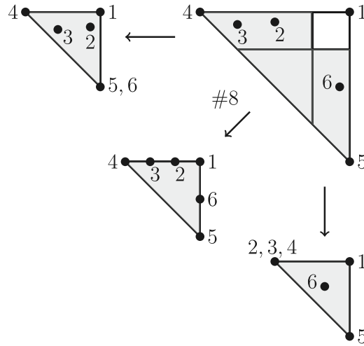
Fig. 12. Maps to the primary components in Example 7.14.
