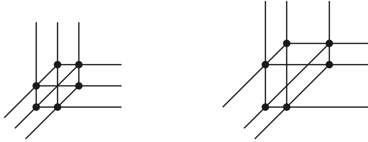
Fig. 5. The lattice classes in \Sigma_{\mathbf{a}} and \Sigma_{\mathbf{b}} in the standard apartment.
