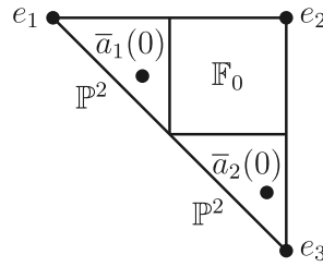
Fig. 13. Fiber of Y_{\mathcal{R}_2} \rightarrow Y_{\mathcal{Q}_2} over \bar{a}(0) in Example 8.11.
