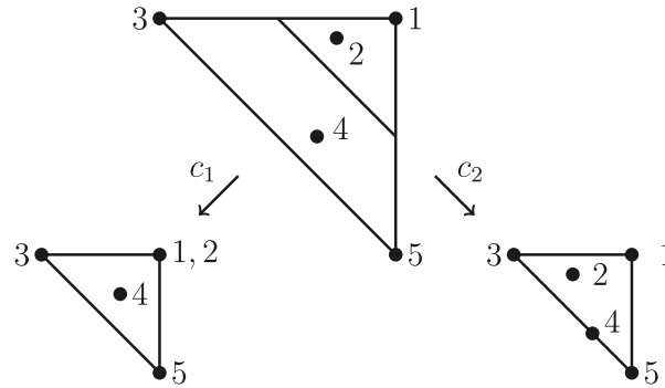
Fig. 9. In red, a fiber of \overline{\mathcal{D}} over a point in \overline{M}_{0,5} (left) and a 0-stratum (right).
