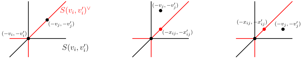
Fig. 19. Possible positions of (-v_j, -v'_j) .
