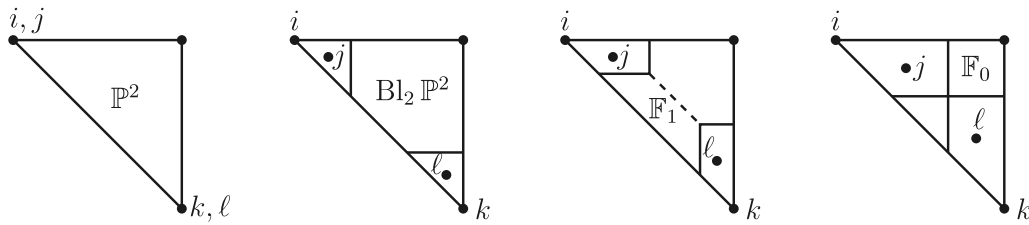
Fig. 8. Fibers of families over the 0-strata.
