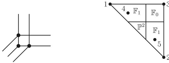
Fig. 4. The lattice classes in \Sigma_{\mathbf{a}} (in the apartment corresponding to the basis e_1, e_2, e_3 ) and the central fiber of the Mustafin join \mathbb{P}(\Sigma_{\mathbf{a}}) of Example 6.2.
