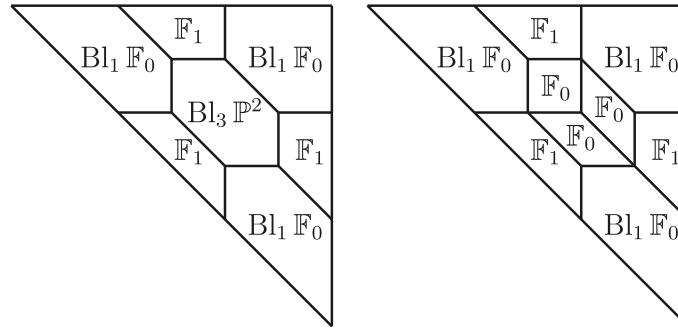
Fig. 5. The lattice classes in \Sigma_{\mathbf{a}} and \Sigma_{\mathbf{b}} in the standard apartment.
