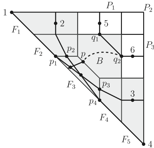
Fig. 22. Cross-ratio \beta in a degeneration of six points in \mathbb{P}^2 parametrized by a point in \bar{X}_{GP}(3,6)^v over the (closed) stratum #23 in \bar{X}(3,6) .
