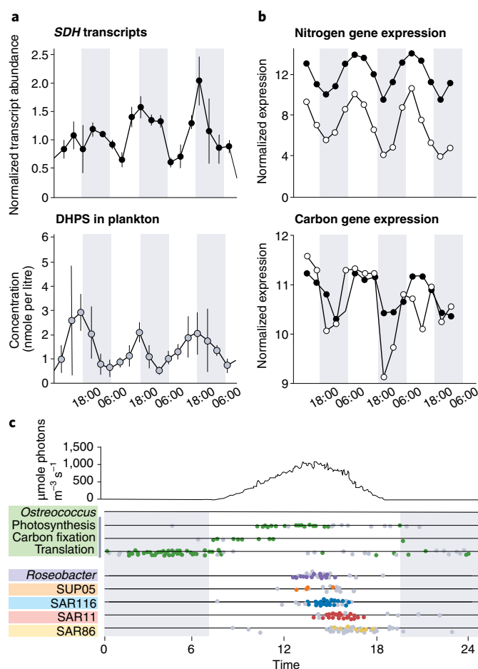
Fig. 3 | Diel synchrony in microbial synthesis, release and utilization of metabolites. a , Periodicity in expression of a diatom gene ( SDH ) in the DHPS biosynthetic pathway (top) is correlated with DHPS concentrations in phytoplankton metabolomes (bottom) in surface waters of the North Pacific Subtropical Gyre. Expression data are transcripts per litre, normalized to the mean. Error bars represent the standard deviation ( n=3 ). Data are from ref. 18 . b , Periodicity in relative gene expression by Trichodesmium (filled symbols) is correlated with expression by its associated microbiome (open symbols) for nitrogen fixation and metabolism genes (top) and carbon fixation and respiration genes (bottom) in the North Atlantic. Data are from ref. 173 . c , Gene expression patterns for key metabolic processes by dominant members of a coastal microbial community in California, averaged over six diel light cycles. Top: photosynthetically active radiation. Bottom: time of peak relative expression for individual genes. Coloured symbols represent genes with statistically significant diel patterns. Gene expression by the dominant primary producer ( Ostreococcus , green symbols) is shown separately for (top to bottom) photosynthesis, carbon fixation and translation. Gene expression by five dominant heterotrophic bacterial groups is shown for translation. Grey shading represents night. Data are from ref. 27 .
