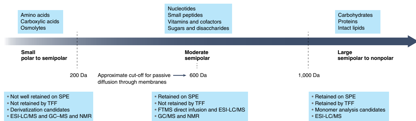
Fig. 4 | The marine DOC spectrum. Chemical analysis strategies for marine DOC are targeted to molecules of different size and hydrophobicity, and typically begin with extraction and concentration from seawater. Solid-phase extraction (SPE) includes common resin types such as C18, C8, hydrophilic-lipophilic balance and priority pollutant. ESI-LC/MS, electrospray ionization-liquid chromatography/MS; FTMS, Fourier transformMS (includes Orbitrap mass spectrometers and Fourier transform ion cyclotron resonance mass spectrometers); GC/MS, gas chromatography/MS.
