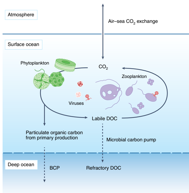
Fig. 1 | Microbial metabolites drive the carbon cycle in the surface ocean.
