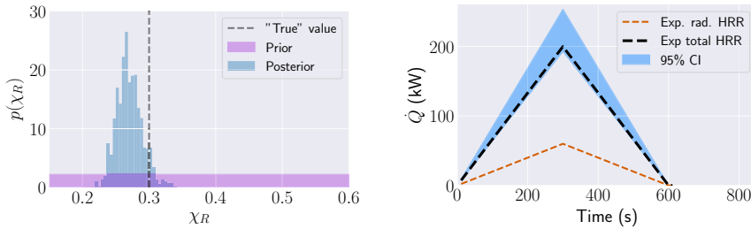
(a) The prior and posterior distributions for the 300 second triangle fire. (b) The 95% credible interval for the total HRR curve implied by the posterior of \chi_R .
