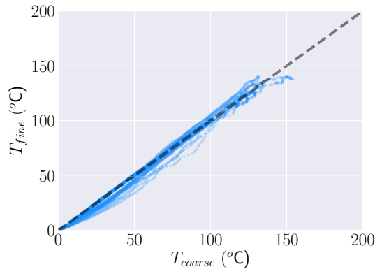
Figure 4. Comparison of FDS results using a 20 cm grid and a 10 cm grid for the t-squared fire ramp shown in Fig. 1. The results are pooled across all 17 thermocouples at all times in the simulation.
