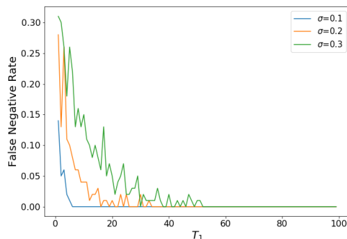
Figure 4. False negative rate of attackability test
