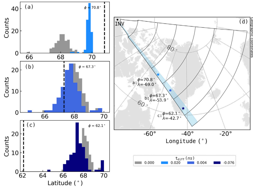
Fig. 2. INV t_{\text{diff}} estimations for the 12.2–12.5 MHz frequency band made along beam 15 using ground scatter with power at or above 1 dB, slant ranges between 3555 km and 4230 km, and times between 1600 and 0400 UT (from the 1–2 June 2016). Panels (a)–(c) show the geolocation results of the t_{\text{diff}} estimation assuming the three different ‘known locations’ from panel (d). In each of the first three panels the black dashed line marks the ‘known’ latitude, the grey histogram shows the geolocation of the data using the hardware t_{\text{diff}} , and the blue histograms show the geolocation of the data using the estimated t_{\text{diff}} . The different shades of blue correspond to different starred locations in panel (d), which are also marked with the corresponding panel letter. (For interpretation of the references to colour in this figure legend, the reader is referred to the web version of this article.)
