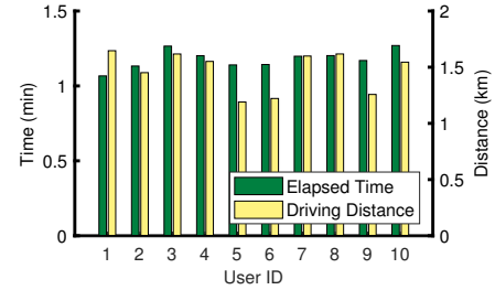
Fig. 13. Average driving time and distance for ten different drivers.
