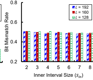
Fig. 10. BMR (stalking attack).
