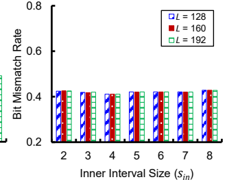
Fig. 11. BMR (measurement attack).
