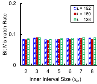
Fig. 8. BMR vs. s_{in} (legitimate).
