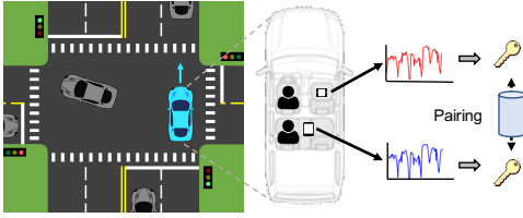
Fig. 1. GPS-equipped devices can use driving data for key establishment.
