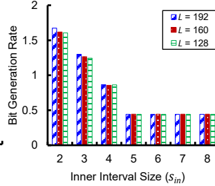
Fig. 9. BGR vs. s_{in} (legitimate).
