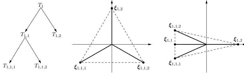
FIG 1. The hierarchical structure (left panel), the embedded points for the standard multicategory classification considering only leaf nodes (middle panel) and the embedded points for hierarchical classification (right panel) of an illustrative example.
