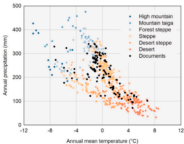
Fig. 6. Locations of studies included in the literature review (black dots) in the climate space, as defined by mean annual temperature (°C) and mean annual precipitation (mm), as extracted from WorldClim (Fick and Hijmans 2017). The colored dots show 500 locations randomly distributed throughout Mongolia; colors indicate different ecological zones. (For interpretation of the references to color in this figure legend, the reader is referred to the Web version of this article.)
