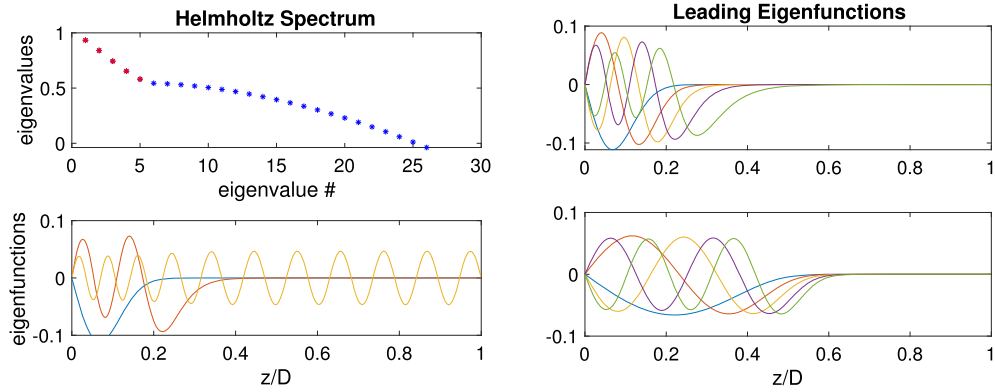
FIG. 3. Left: The figure illustrates the spectrum of the one-dimensional Schrödinger operator associated with the background index of refraction profile when D is finite and d/D \approx .2 . The top plot shows the normalized eigenvalues \gamma_i / (n_0 k)^2 . There are 5 surface modes indicated by the red stars. The bottom plot shows eigenfunctions 1, 4 and 20. The modes 1 and 4 correspond to surface modes and are supported essentially in the surface layer, while the mode 20 corresponds to a body mode and is oscillatory and is supported in the full waveguide. Right: The top plot shows the first 5 eigenfunctions corresponding to the background profile shown in Fig. 1 when d/D \approx .2 . The bottom plot shows the corresponding eigenfunctions when the width of the surface layer is tripled till d/D \approx .6 , and we see that the support of the eigenfunctions has been correspondingly extended
