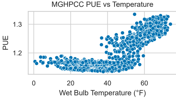
Fig. 2. PUE of the MGHPCC data center as a function of outdoor wet bulb temperature.
