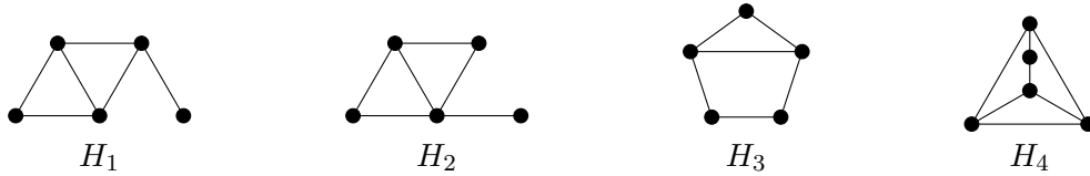
Figure 3: Wolf’s list of 5-vertex connected graphs that were not known to be (un)common in 2017.
