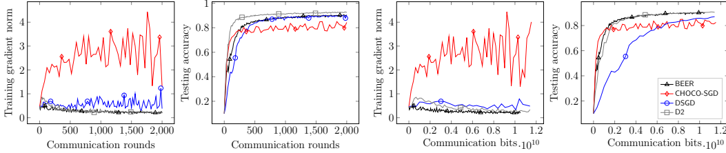
Figure 2: The training gradient norm and testing accuracy against communication rounds (left two panels) and communication bits (right two panels) for classification on unshuffled MNIST dataset using a 1-hidden-layer neural network. Both BEER and CHOCO-SGD employ the biased \text{gsgd}_b compression [1] with b = 20 .
