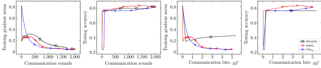
Figure 5: The training gradient norm and testing accuracy against communication rounds (left two panels) and communication bits (right two panels) for BEER using different compression algorithms on logistic regression with nonconvex regularization on unshuffled a9a dataset.
