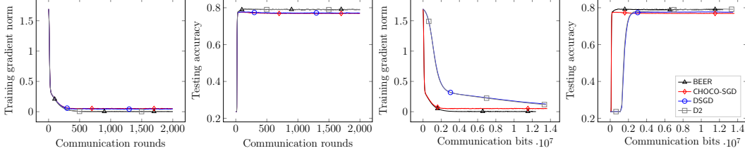
Figure 1: The training gradient norm and testing accuracy against communication rounds (left two panels) and communication bits (right two panels) for logistic regression with nonconvex regularization on unshuffled a9a dataset. Both BEER and CHOCO-SGD employ the biased \text{gsgd}_b compression [1] with b = 5 .
