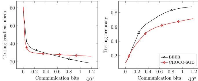
Figure 3: The testing gradient norm and testing accuracy against communication bits on unshuffled MNIST dataset using a 3-layer convolutional neural network. Both BEER and CHOCO-SGD employ the biased \text{gsgd}_b compression [1] with b = 5 .
