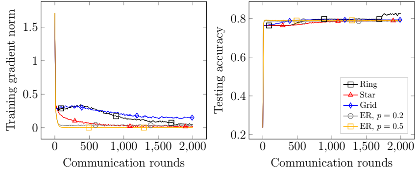
Figure 4: The training gradient norm and testing accuracy against communication rounds for BEER using biased \text{gsgd}_b compression [1] with b = 5 on logistic regression with nonconvex regularization on unshuffled a9a dataset.
