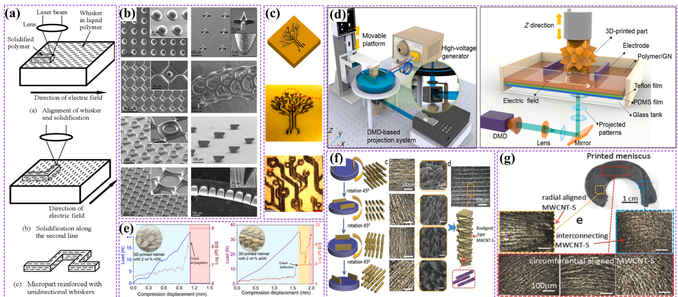
Fig. 12. Electric field-assisted extrusion-based AM: a) Schematic of filler alignment using electric field in laser stereolithography [293]. b) Piezoelectric microstructures built by digital projection printing (right column) and 3D structures manufactured by dynamic optical projection stereolithography (left column) [294]. c) CAD model, 3D view, and microscopic image of part manufactured by projection electro-stereolithography [296]. d) Illustration of the electric field-assisted additive manufacturing process and the SLA setup used for this purpose [301]. e) 3D printed composites of random and aligned graphene nanoplatelets show different behaviors, complete disconnection vs. self-healing properties, under compression tests and simultaneous electrical potential [301]. f) Schematic, SEM, and surface optical microscopic images of MWCNTs in 3D printed to mimic natural materials [300]. g) Electric field-assisted additive manufacturing is used to build an artificial meniscus with selective alignment of MWCNTs in different areas [300].
