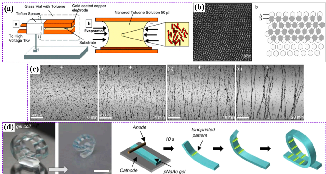
Fig. 13. Electric field-assisted alignment in conventional manufacturing processes: a) schematic of the filler alignment using electric-field-assisted assembly [303]. b) Nanorods of cadmium sulfide (CdS) are aligned in 3D and deposited under electric field [303]. c) Application of electric field to graphene nanoparticles suspended in epoxy resins leads to orienting the particles in the time span of 20 s [306]. d) Unfolding a 3D gel coil by ionprinted lines and recovery to its original shape by dehydration [307].
