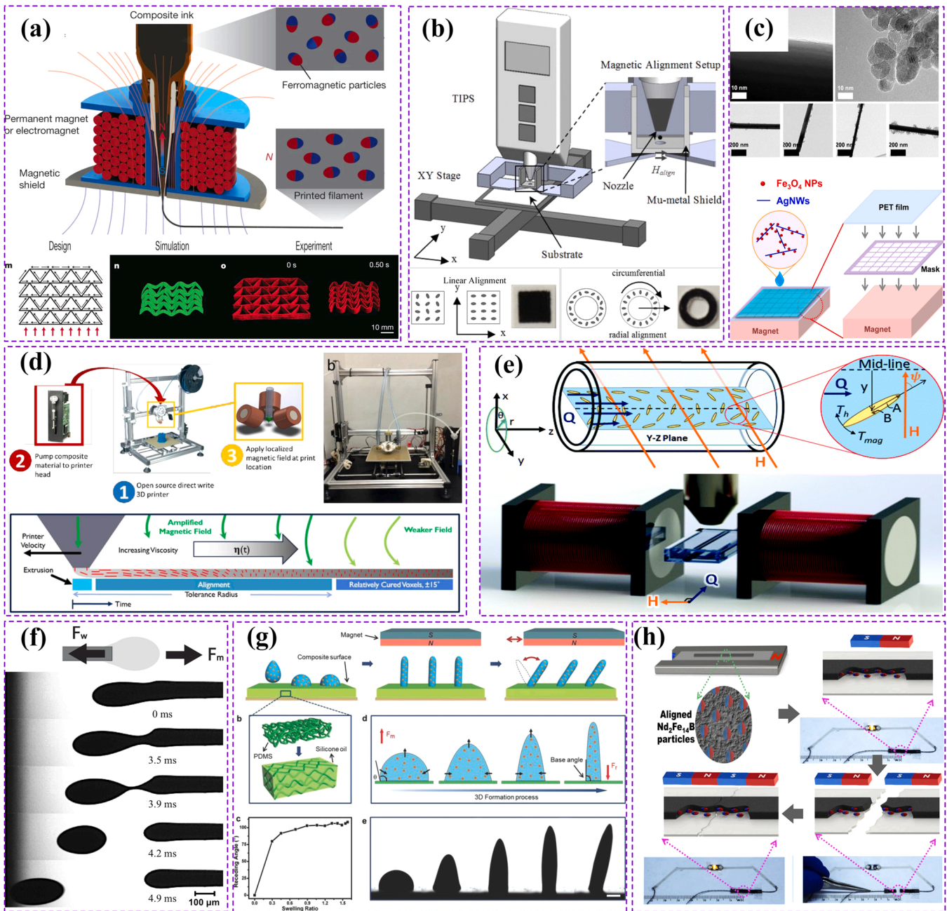
Fig. 8. Magnetic field-assisted extrusion-based AM: a) Example of using magnetic field during the extrusion process to print magnetic domains and build smart and functional structures [186]. b) Example of using magnetic field after extrusion of the material to align particles in different directions [189]. c) 3D printing and magnetic patterning of silver nanowires [190]. d) Extrusion-based magnetic AM to align particles and their real-time orientation [192]. e) Extrusion setup and schematic basis of studying the magnetic torque for fiber alignment [196]. f) Force balancing during the magnetic droplet manipulation for 3D printing purposes [36]. g) Precise microstructures controlled by magnetic field [200]. h) Self-healing structures by magnetic alignment after printing [201].
