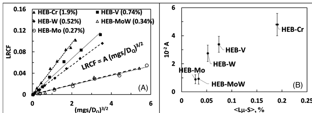
FIGURE 7 (A) Linearization of the long-range chemical fluctuation (LRCF) data versus \text{mgs}/D_Q according to the power law \text{LRCF} = A (\text{mgs}/D_Q)^{3/2} ; (B) the A parameter versus average lattice \mu -strain \langle L\mu-S \rangle
