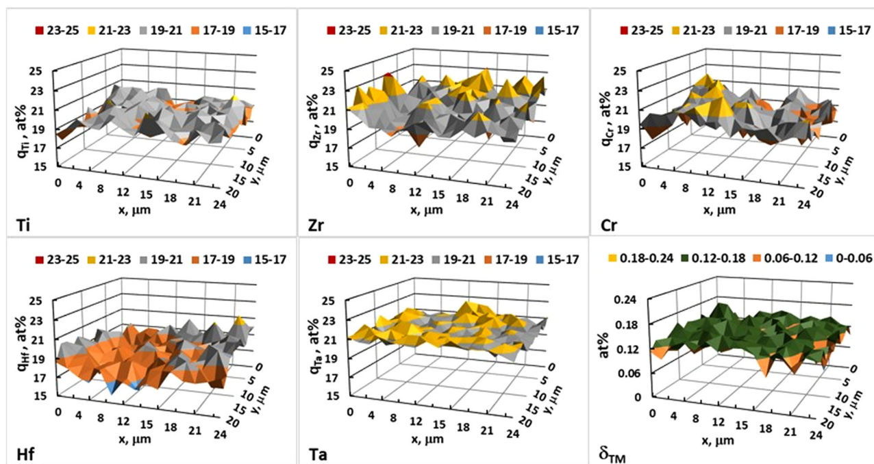
FIGURE 8 Quantitative mapping of HEB-Cr with the atomic percent q_{\text{TM}} of various metals (TM) versus linear dimension (x, y) of the mapped area, \Sigma q_{\text{TM}} = 100\% . The corresponding \delta_{\text{TM}} descriptor is shown: note that it has a different colored palette than the TM constituents
