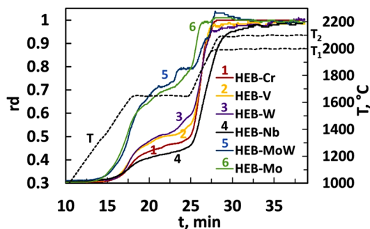
FIGURE 3 Relative density (rd) versus time ( t ) calculated using relation (1): the second dwell was set at T_1 = 2000^\circ\text{C} (curves 1,5,6) or T_2 = 2100^\circ\text{C} (curves 2,3,4)
