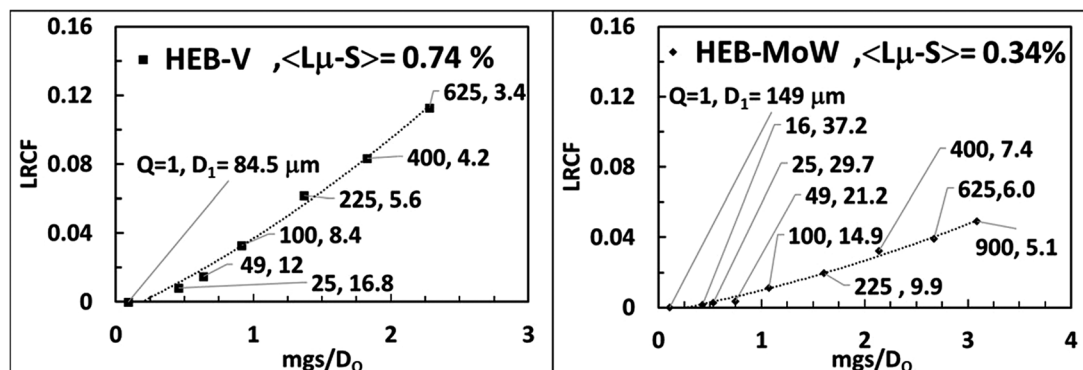
FIGURE 6 Long-range chemical fluctuations (LRCF) versus \text{mgs}/D_Q in HEB-V and HEB-MoW as examples showing the Q - D_Q pairs (cfr. Equation (1)) for each experimental point: the D_Q unit in \mu\text{m} is omitted for Q > 1 . The average lattice \mu -strains \langle L\mu-S \rangle are also indicated
