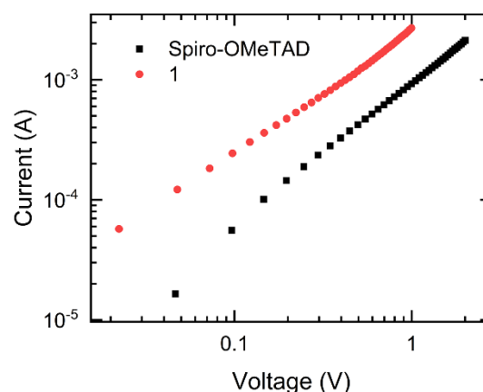
Fig. 5 Current(I) - Voltage (V) characteristics of Spiro-OMeTAD, and 1 .
