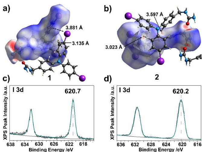
Fig. 3 Hirshfeld surface map (Isovalue 0.05) and I(3d) XPS core level peaks recorded with a monochromatic Al Kα X-ray source of the asymmetric unit of 1 and 2 . a) Hirshfeld surface map of 1 showing C-I...π, and offset π stacking interactions. b) Hirshfeld surface map of 2 showing offset π stacking interactions. c) I(3d) XPS core level peaks for 1 (ethyl acetate solvated). d) I(3d) XPS core level peaks for 2 .
