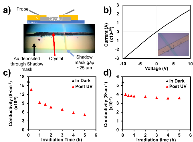
Fig. 4 Electrical conductivity measurement under dark and UV-irradiation at room temperature. a) two contact probe setup used to measure the conductivity of a single crystal (shadow mask gap 25 μm). b) I-V curve for a trial of 1 under dark at room temperature by measuring the sum of resistance of the material, wires, and contacts using two contact probe method. Inset shows a single crystal setup. c, d) changes in electrical conductivity under UV-irradiation using 365 nm UV sources at room temperature for 1 and 2 respectively.
