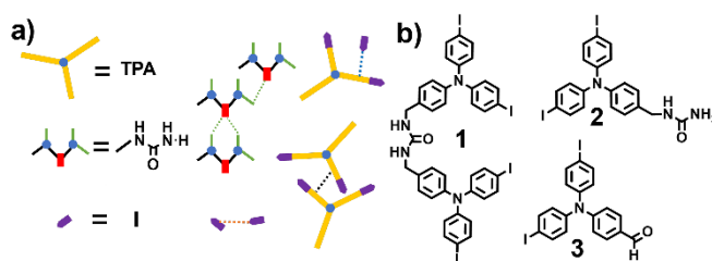
Fig. 1 a) Schematic of non-covalent interactions for organizing linear triphenylamine (TPA) include intra/intermolecular hydrogen bond (green), I-I halogen bond (orange), I- \pi interactions (blue), offset \pi - \pi stacking interaction (black). b) Comparison of TPA structures investigated. TPA tethered to both side of urea 1 . TPA tethered to one side of urea 2 . TPA 3 lacking the urea assembly motif.
