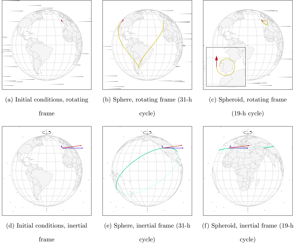
FIG. 1. CorioVis snapshots of one cycle of the periodic motion of a puck that slides without friction on a sphere and a stably rotating spheroid whose volumes, angular speeds of rotation, and flattening (for the spheroid) match the earth's. As viewed in the rotating frame, the puck is projected northward from latitude 40^\circ at 50 m/s, a speed that is comparable to the fastest measured ice hockey slapshot (a). 26,27 As viewed in the inertial frame, the puck's initial velocity is 360 m/s toward the northeast, including a large eastward component due to the earth's rotation (d). On the sphere ( CorioVis 28 Demo 1), the motion resulting from these initial conditions has period 31 h and consists of zigzag motion at a variable speed in the rotating frame (b) and motion on a great circle at a constant speed of 360 m/s in the inertial frame (e). On the spheroid ( CorioVis 28 Demo 2), the motion resulting from these initial conditions has period 19 h and consists of clockwise inertial oscillations at a constant speed of 50 m/s in the rotating frame (c) and incomplete orbits at a variable speed in the inertial frame (f). Blue arrows that point eastward and northward represent velocity components in these directions, and red arrows that point in the direction of motion represent velocity vectors.
