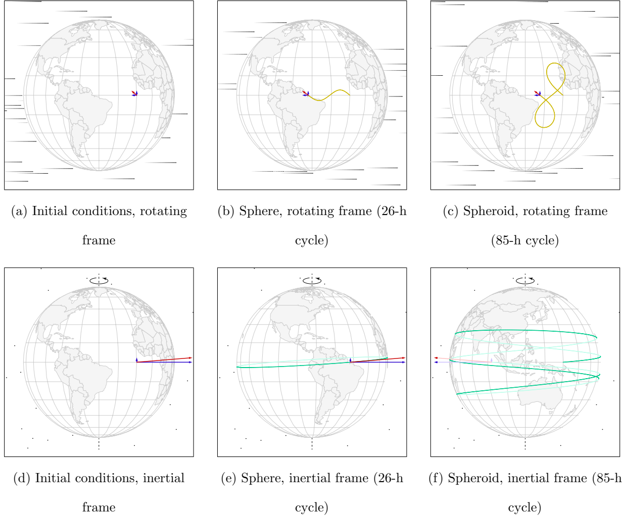
FIG. 4. CorioVis snapshots of one cycle of the periodic motion on spherical and stably rotating spheroidal earths for a puck projected northwest from the equator at 50 m/s in the rotating frame (a). As seen by an observer in the inertial frame, the puck's initial velocity is 426 m/s toward the northeast, and includes a large eastward component due to the earth's rotation (d). On the sphere ( CorioVis 28 Demo 3), the motion resulting from these initial conditions has period 26 h and consists of sinusoidal motion at a variable speed in the rotating frame (b) and motion on a great circle at a constant speed of 426 m/s in the inertial frame (e). On the spheroid ( CorioVis 28 Demo 4), the motion resulting from these initial conditions has period 85 h and consists of inertial loops at a constant speed of 50 m/s in the rotating frame (c) and multiple orbits at a variable speed in the inertial frame (f). Blue arrows that point eastward and northward represent velocity components in these directions, and red arrows that point in the direction of motion represent velocity vectors.
