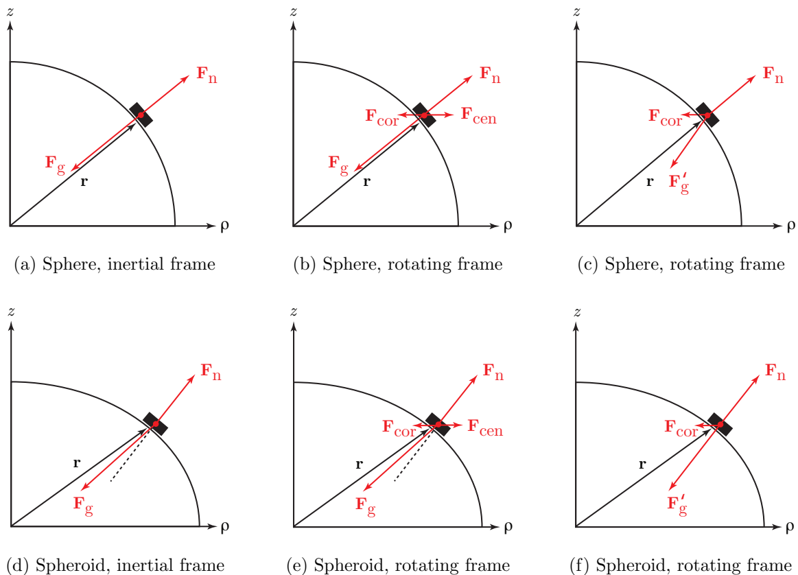
FIG. 3. Free-body diagrams showing the forces acting on a puck that slides without friction on a rotating spherical earth (a-c) and a stably rotating spheroidal earth (d-f, with exaggerated flattening), as seen by observers in the inertial (a, d) and rotating (b, c, e, f) frames. Shown are the gravitational and normal forces \mathbf{F}_g and \mathbf{F}_n that apply in both frames; the Coriolis and centrifugal forces \mathbf{F}_{\text{cor}} and \mathbf{F}_{\text{cen}} that apply only in the rotating frame; and the apparent gravitational force, \mathbf{F}'_g = \mathbf{F}_g + \mathbf{F}_{\text{cen}} , which replaces \mathbf{F}_g and \mathbf{F}_{\text{cen}} in panels (c, f). The gravitational force \mathbf{F}_g is normal to the surface of the sphere (a, b) and the apparent gravitational force \mathbf{F}'_g is normal to the surface of the stably rotating spheroid (f). The dotted line is normal to the spheroid. The Coriolis force is zero for a stationary puck, and is shown in a direction that corresponds to westward motion of the puck (directed out of the plane of the figure).
